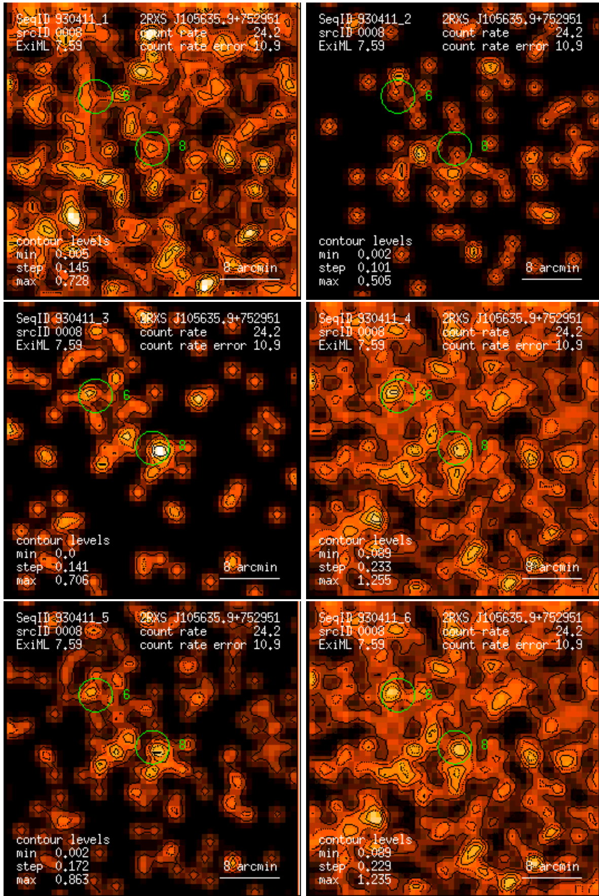
Figure 8: RASS 930411: detection 0008: band rate images, Gaussian filter: (1) PSPC channels 11 – 41, (2) 52 – 90, (3) 91 – 201, (4) 11 – 235, (5) 52 – 201, (6) 11 – 201. Broad band rates in counts/ks. Band rate contour levels in counts/ks/arcmin 2 .
