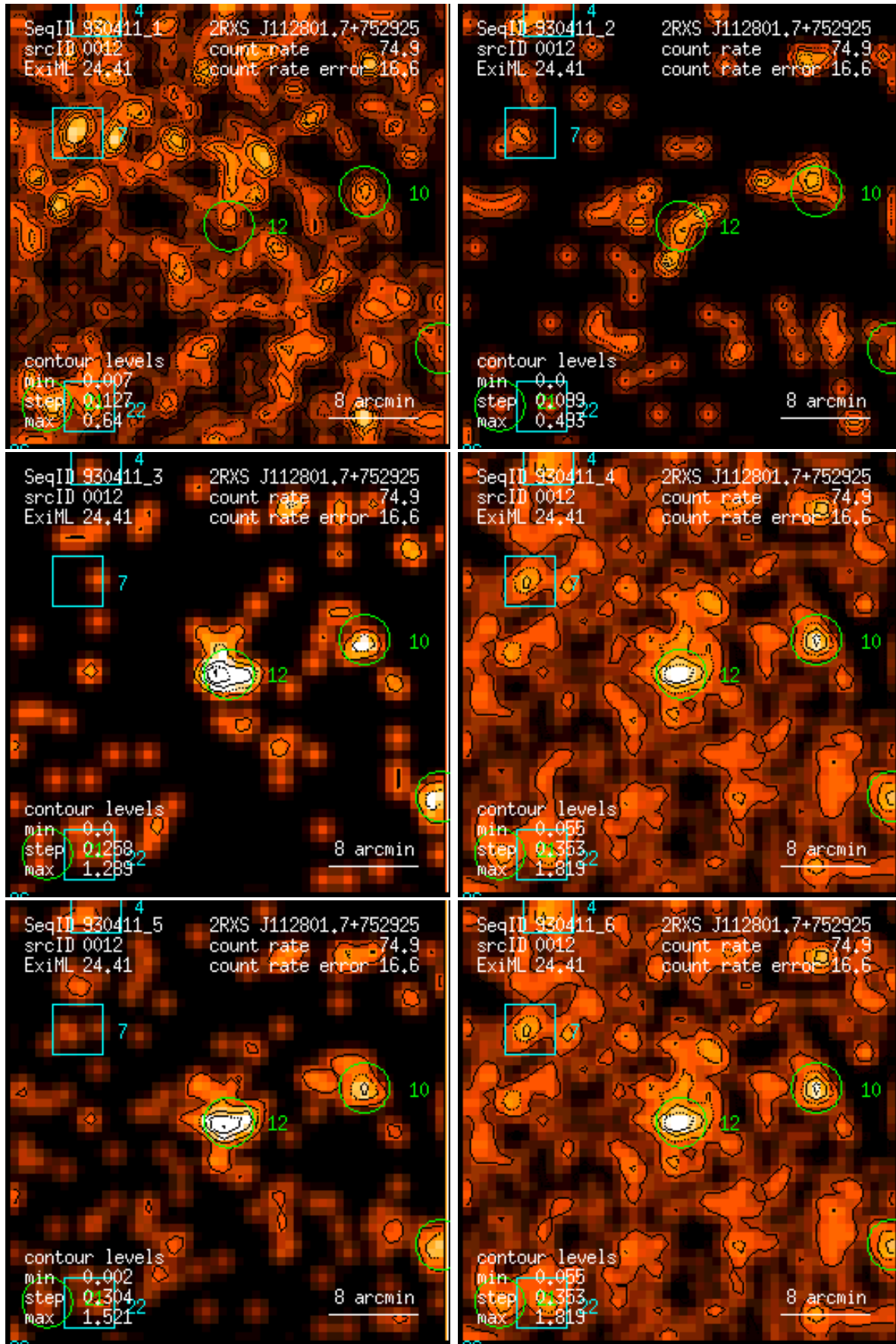
Figure 12: RASS 930411: detection 0012: band rate images, Gaussian filter: (1) PSPC channels 11 – 41, (2) 52 – 90, (3) 91 – 201, (4) 11 – 235, (5) 52 – 201, (6) 11 – 201. Broad band rates in counts/ks. Band rate contour levels in counts/ks/arcmin 2 .
