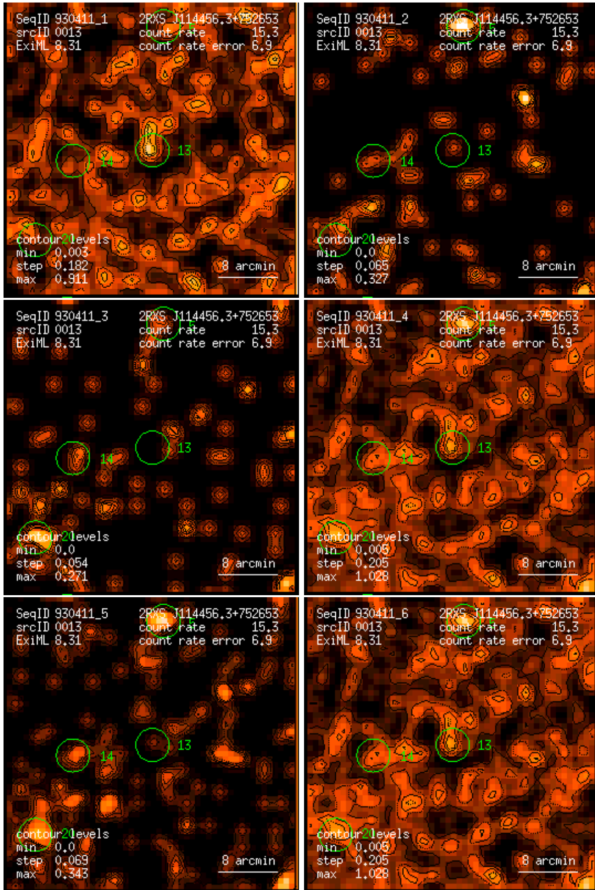
Figure 13: RASS 930411: detection 0013: band rate images, Gaussian filter: (1) PSPC channels 11 – 41, (2) 52 – 90, (3) 91 – 201, (4) 11 – 235, (5) 52 – 201, (6) 11 – 201. Broad band rates in counts/ks. Band rate contour levels in counts/ks/arcmin 2 .
