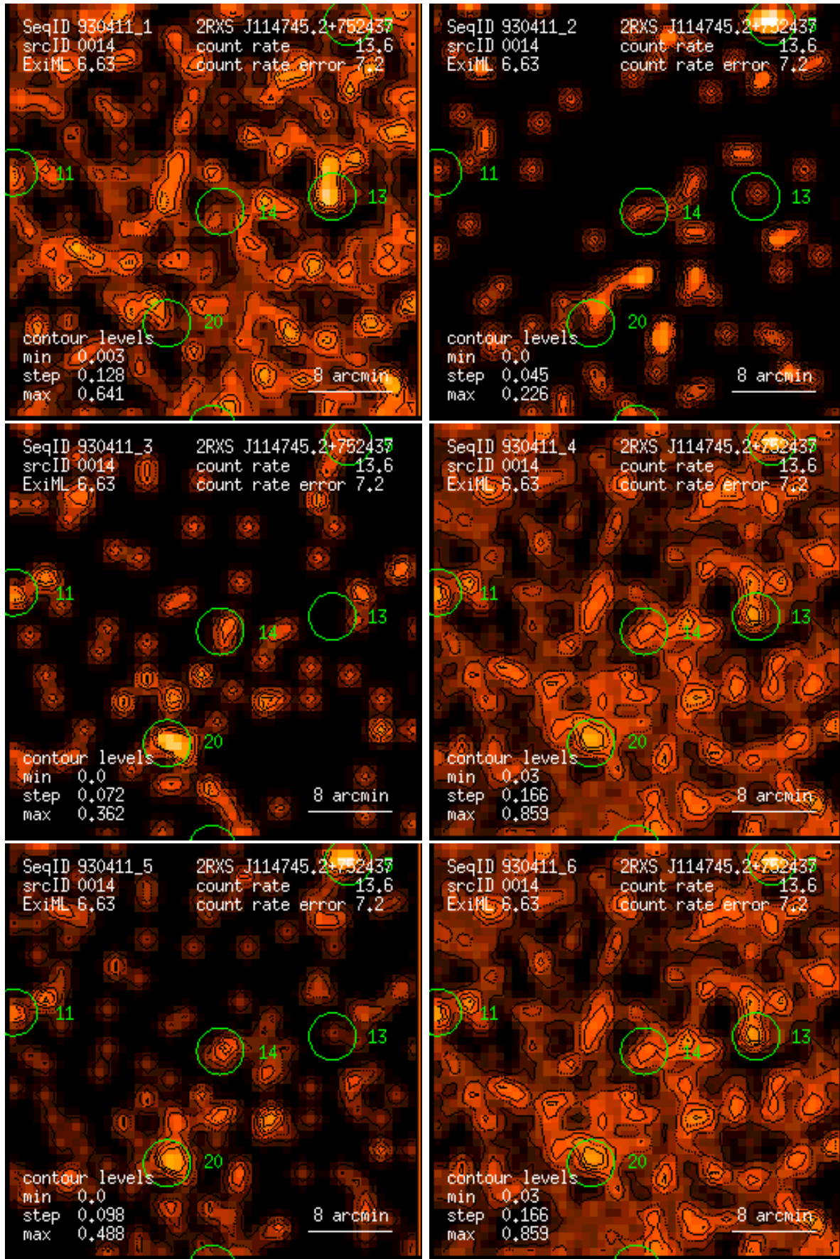
Figure 14: RASS 930411: detection 0014: band rate images, Gaussian filter: (1) PSPC channels 11 – 41, (2) 52 – 90, (3) 91 – 201, (4) 11 – 235, (5) 52 – 201, (6) 11 – 201. Broad band rates in counts/ks. Band rate contour levels in counts/ks/arcmin 2 .
