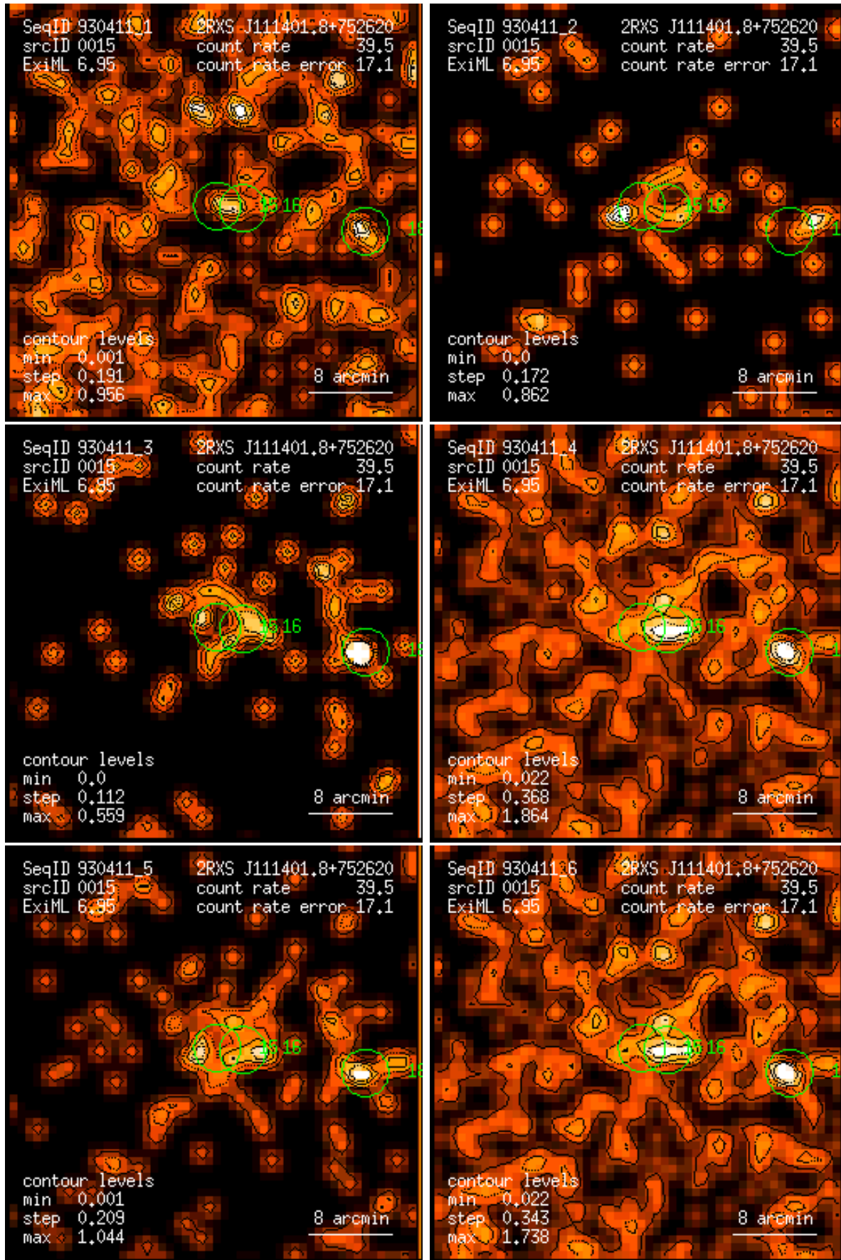
Figure 15: RASS 930411: detection 0015: band rate images, Gaussian filter: (1) PSPC channels 11 – 41, (2) 52 – 90, (3) 91 – 201, (4) 11 – 235, (5) 52 – 201, (6) 11 – 201. Broad band rates in counts/ks. Band rate contour levels in counts/ks/arcmin 2 .
