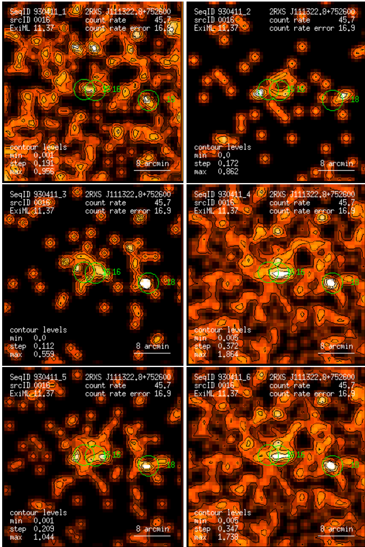
Figure 16: RASS 930411: detection 0016: band rate images, Gaussian filter: (1) PSPC channels 11 – 41, (2) 52 – 90, (3) 91 – 201, (4) 11 – 235, (5) 52 – 201, (6) 11 – 201. Broad band rates in counts/ks. Band rate contour levels in counts/ks/arcmin 2 .
