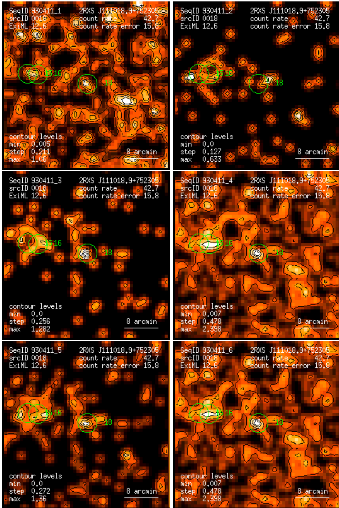
Figure 18: RASS 930411: detection 0018: band rate images, Gaussian filter: (1) PSPC channels 11 – 41, (2) 52 – 90, (3) 91 – 201, (4) 11 – 235, (5) 52 – 201, (6) 11 – 201. Broad band rates in counts/ks. Band rate contour levels in counts/ks/arcmin 2 .
