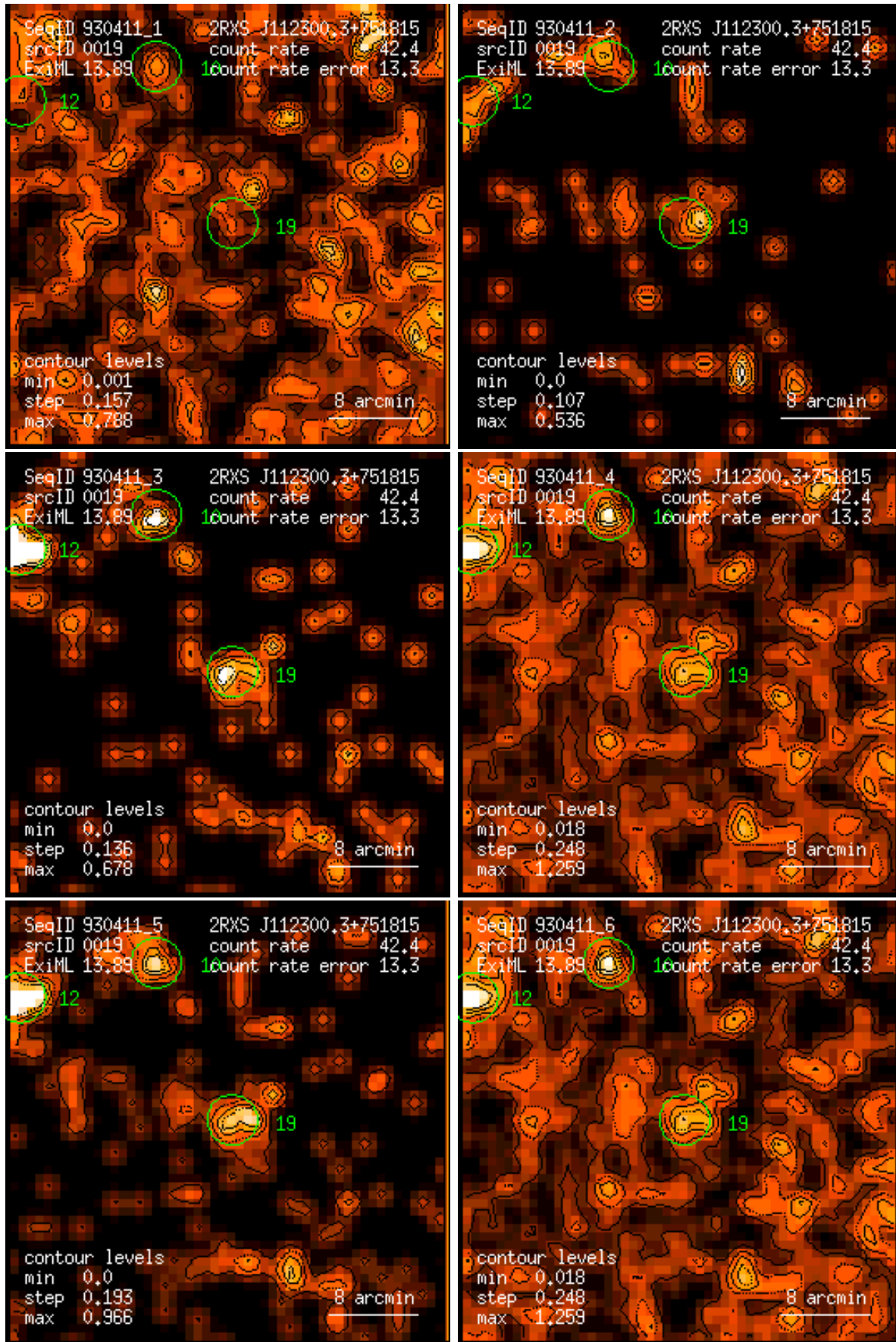
Figure 19: RASS 930411: detection 0019: band rate images, Gaussian filter: (1) PSPC channels 11 – 41, (2) 52 – 90, (3) 91 – 201, (4) 11 – 235, (5) 52 – 201, (6) 11 – 201. Broad band rates in counts/ks. Band rate contour levels in counts/ks/arcmin 2 .
