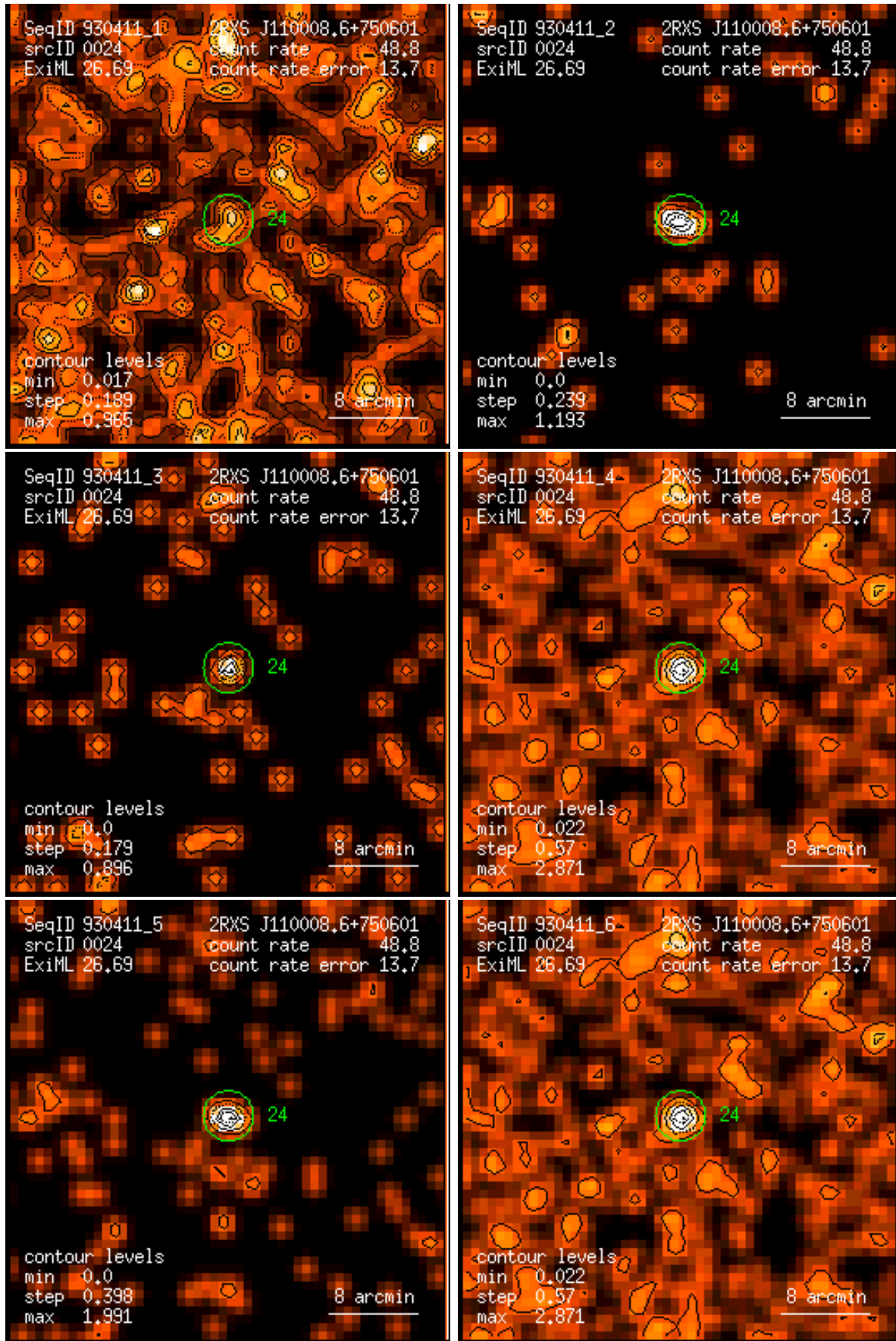
Figure 24: RASS 930411: detection 0024: band rate images, Gaussian filter: (1) PSPC channels 11 – 41, (2) 52 – 90, (3) 91 – 201, (4) 11 – 235, (5) 52 – 201, (6) 11 – 201. Broad band rates in counts/ks. Band rate contour levels in counts/ks/arcmin 2 .
