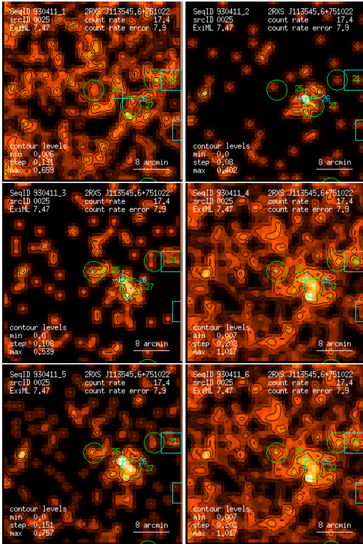
Figure 25: RASS 930411: detection 0025: band rate images, Gaussian filter: (1) PSPC channels 11 – 41, (2) 52 – 90, (3) 91 – 201, (4) 11 – 235, (5) 52 – 201, (6) 11 – 201. Broad band rates in counts/ks. Band rate contour levels in counts/ks/arcmin 2 .
