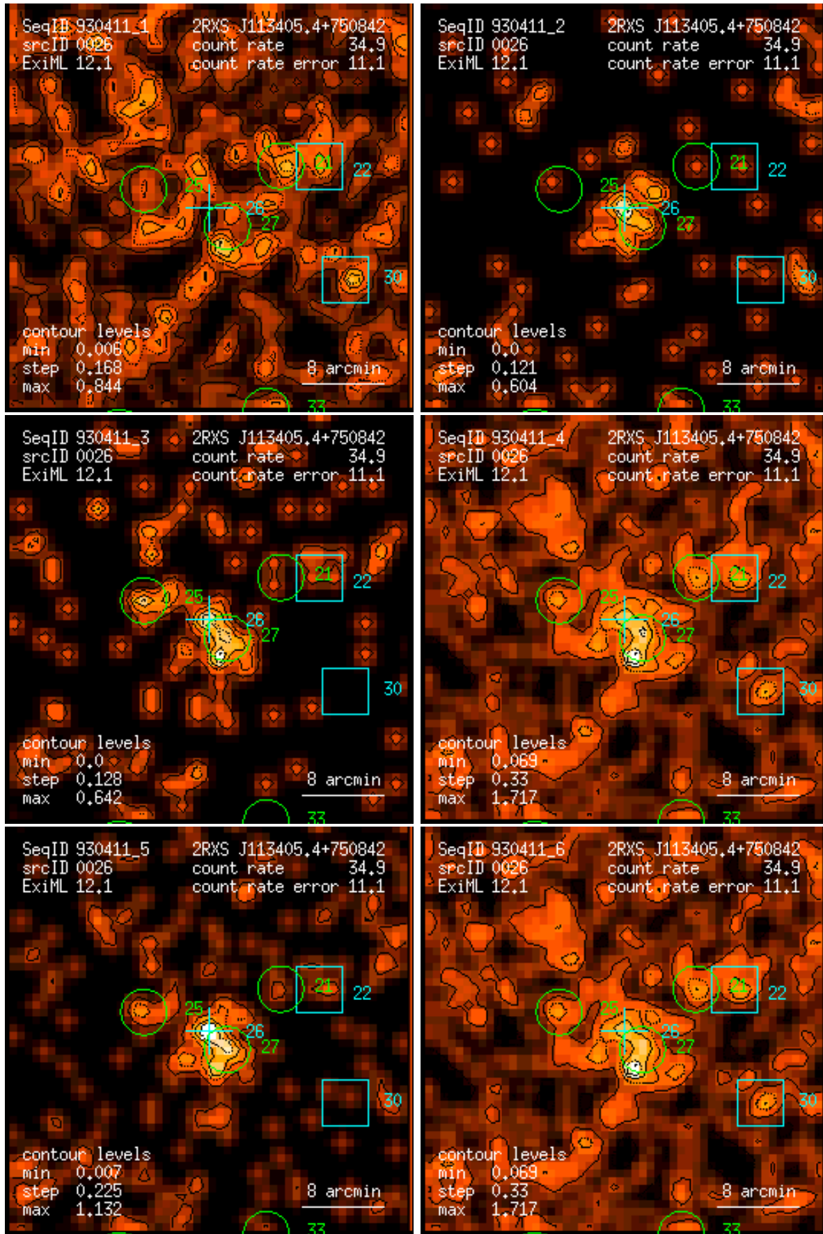
Figure 26: RASS 930411: detection 0026: band rate images, Gaussian filter: (1) PSPC channels 11 – 41, (2) 52 – 90, (3) 91 – 201, (4) 11 – 235, (5) 52 – 201, (6) 11 – 201. Broad band rates in counts/ks. Band rate contour levels in counts/ks/arcmin 2 .
