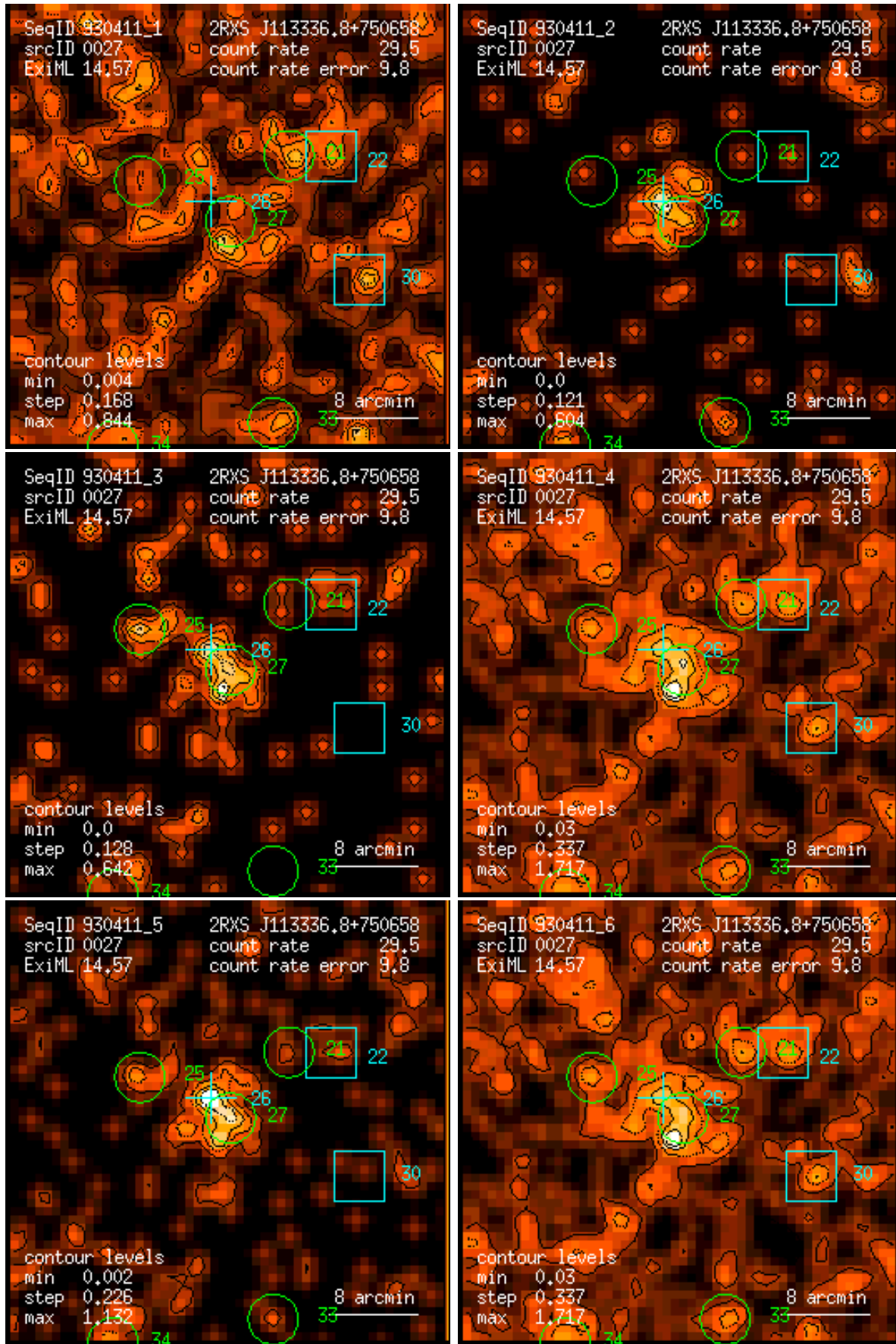
Figure 27: RASS 930411: detection 0027: band rate images, Gaussian filter: (1) PSPC channels 11 – 41, (2) 52 – 90, (3) 91 – 201, (4) 11 – 235, (5) 52 – 201, (6) 11 – 201. Broad band rates in counts/ks. Band rate contour levels in counts/ks/arcmin 2 .
