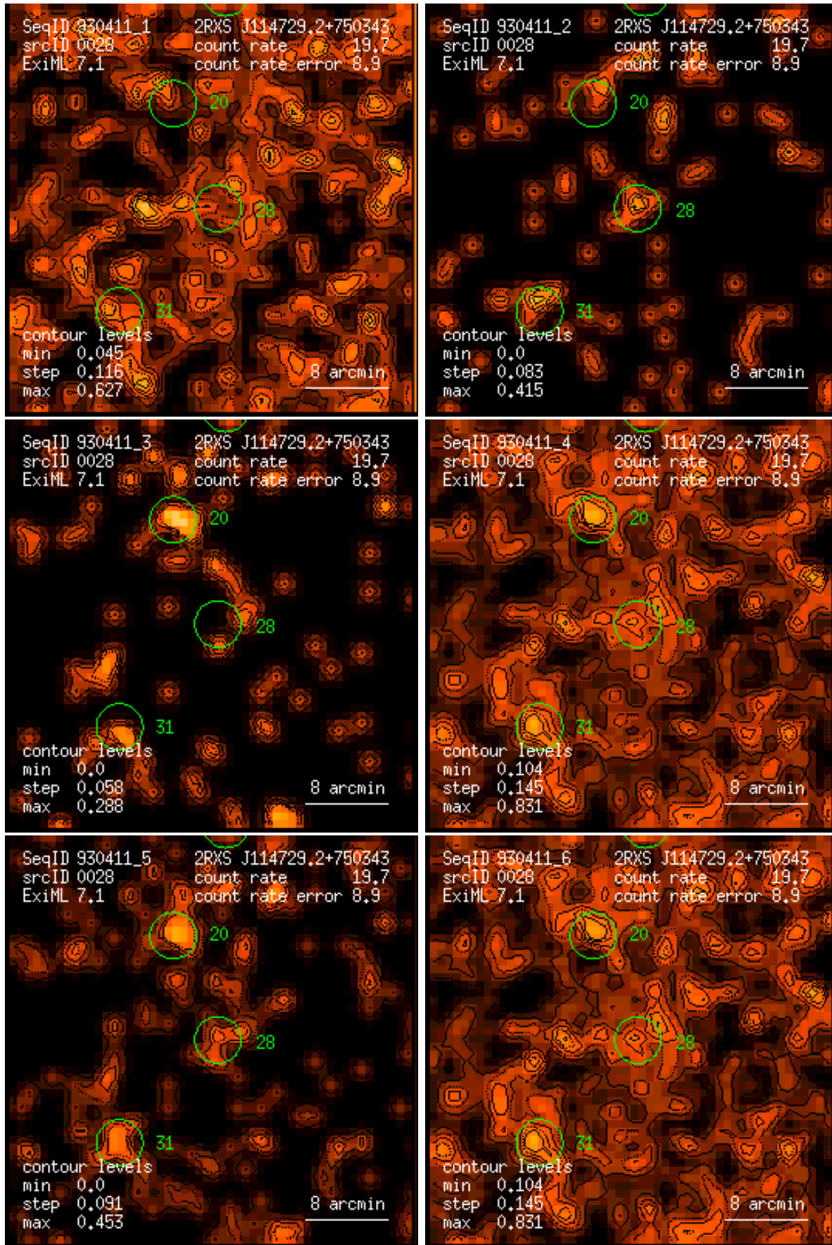
Figure 28: RASS 930411: detection 0028: band rate images, Gaussian filter: (1) PSPC channels 11 – 41, (2) 52 – 90, (3) 91 – 201, (4) 11 – 235, (5) 52 – 201, (6) 11 – 201. Broad band rates in counts/ks. Band rate contour levels in counts/ks/arcmin 2 .
