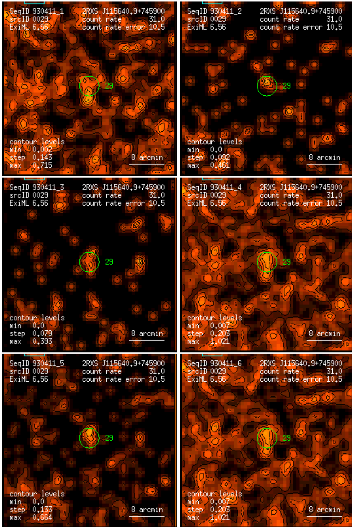
Figure 29: RASS 930411: detection 0029: band rate images, Gaussian filter: (1) PSPC channels 11 – 41, (2) 52 – 90, (3) 91 – 201, (4) 11 – 235, (5) 52 – 201, (6) 11 – 201. Broad band rates in counts/ks. Band rate contour levels in counts/ks/arcmin 2 .
