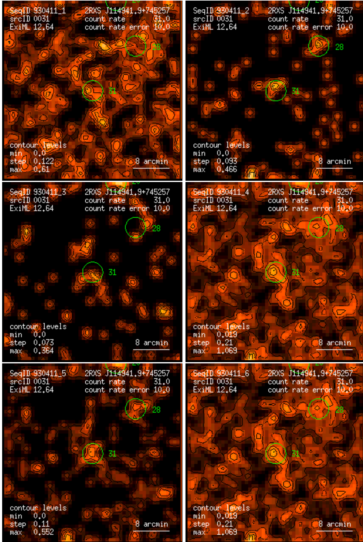
Figure 31: RASS 930411: detection 0031: band rate images, Gaussian filter: (1) PSPC channels 11 – 41, (2) 52 – 90, (3) 91 – 201, (4) 11 – 235, (5) 52 – 201, (6) 11 – 201. Broad band rates in counts/ks. Band rate contour levels in counts/ks/arcmin 2 .
