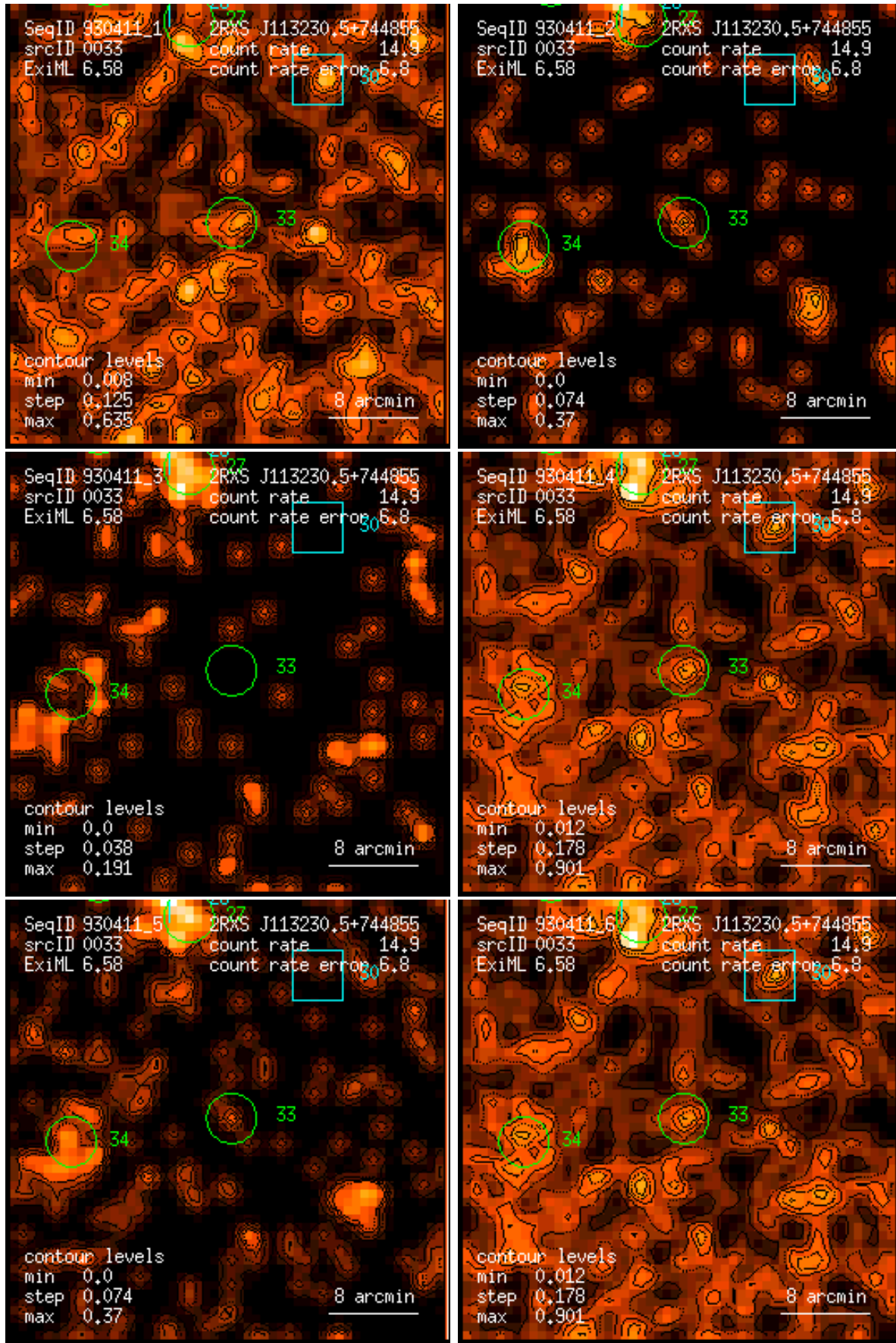
Figure 33: RASS 930411: detection 0033: band rate images, Gaussian filter: (1) PSPC channels 11 – 41, (2) 52 – 90, (3) 91 – 201, (4) 11 – 235, (5) 52 – 201, (6) 11 – 201. Broad band rates in counts/ks. Band rate contour levels in counts/ks/arcmin 2 .
