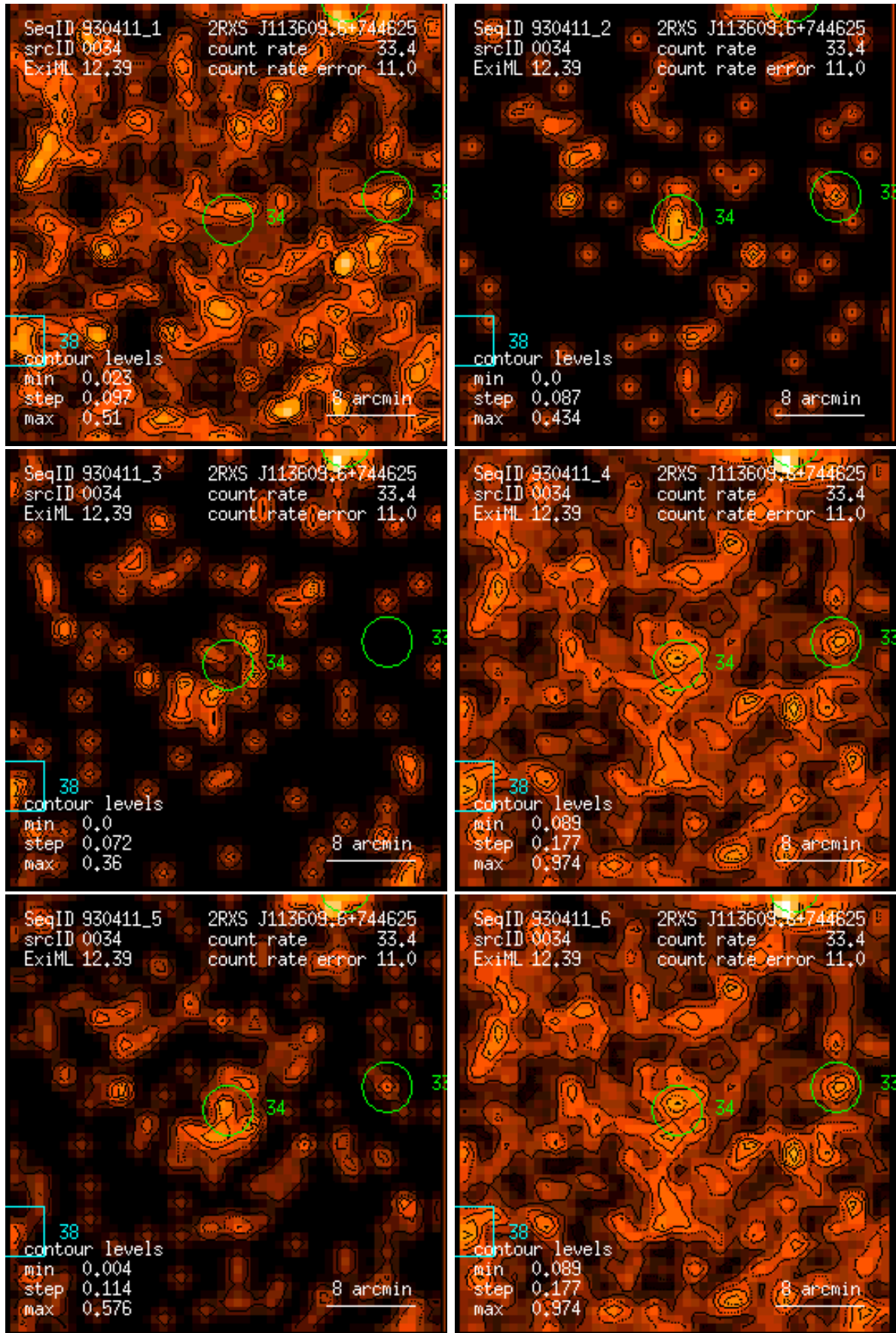
Figure 34: RASS 930411: detection 0034: band rate images, Gaussian filter: (1) PSPC channels 11 – 41, (2) 52 – 90, (3) 91 – 201, (4) 11 – 235, (5) 52 – 201, (6) 11 – 201. Broad band rates in counts/ks. Band rate contour levels in counts/ks/arcmin 2 .
