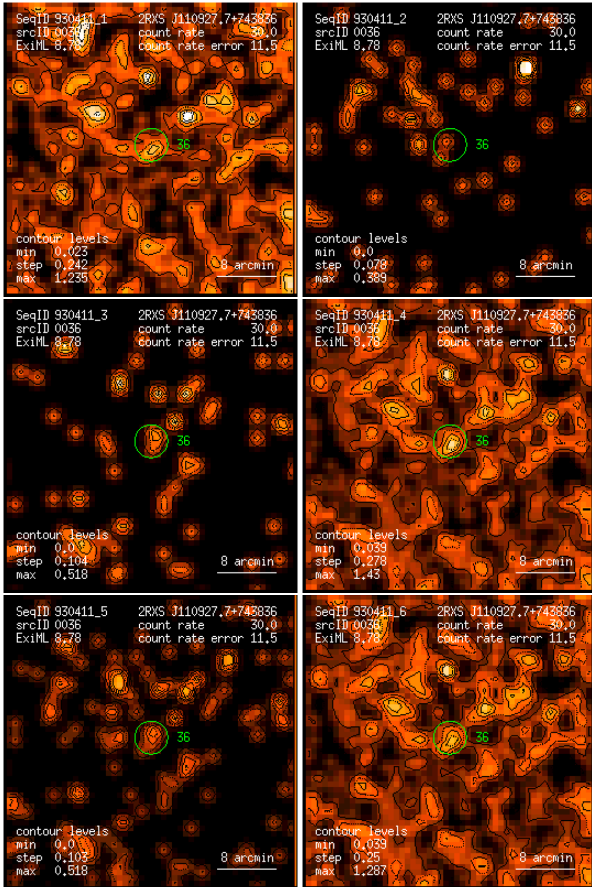
Figure 36: RASS 930411: detection 0036: band rate images, Gaussian filter: (1) PSPC channels 11 – 41, (2) 52 – 90, (3) 91 – 201, (4) 11 – 235, (5) 52 – 201, (6) 11 – 201. Broad band rates in counts/ks. Band rate contour levels in counts/ks/arcmin 2 .
