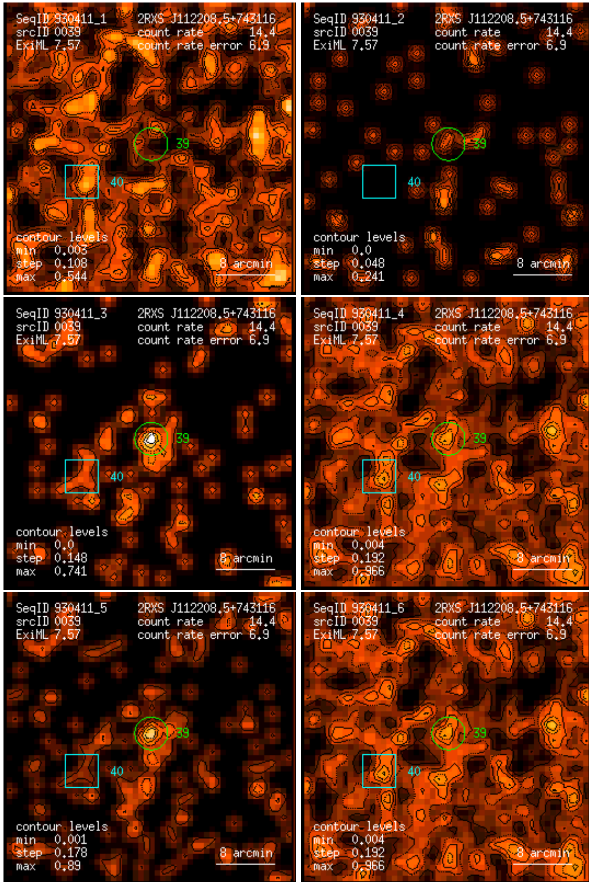
Figure 39: RASS 930411: detection 0039: band rate images, Gaussian filter: (1) PSPC channels 11 – 41, (2) 52 – 90, (3) 91 – 201, (4) 11 – 235, (5) 52 – 201, (6) 11 – 201. Broad band rates in counts/ks. Band rate contour levels in counts/ks/arcmin 2 .
