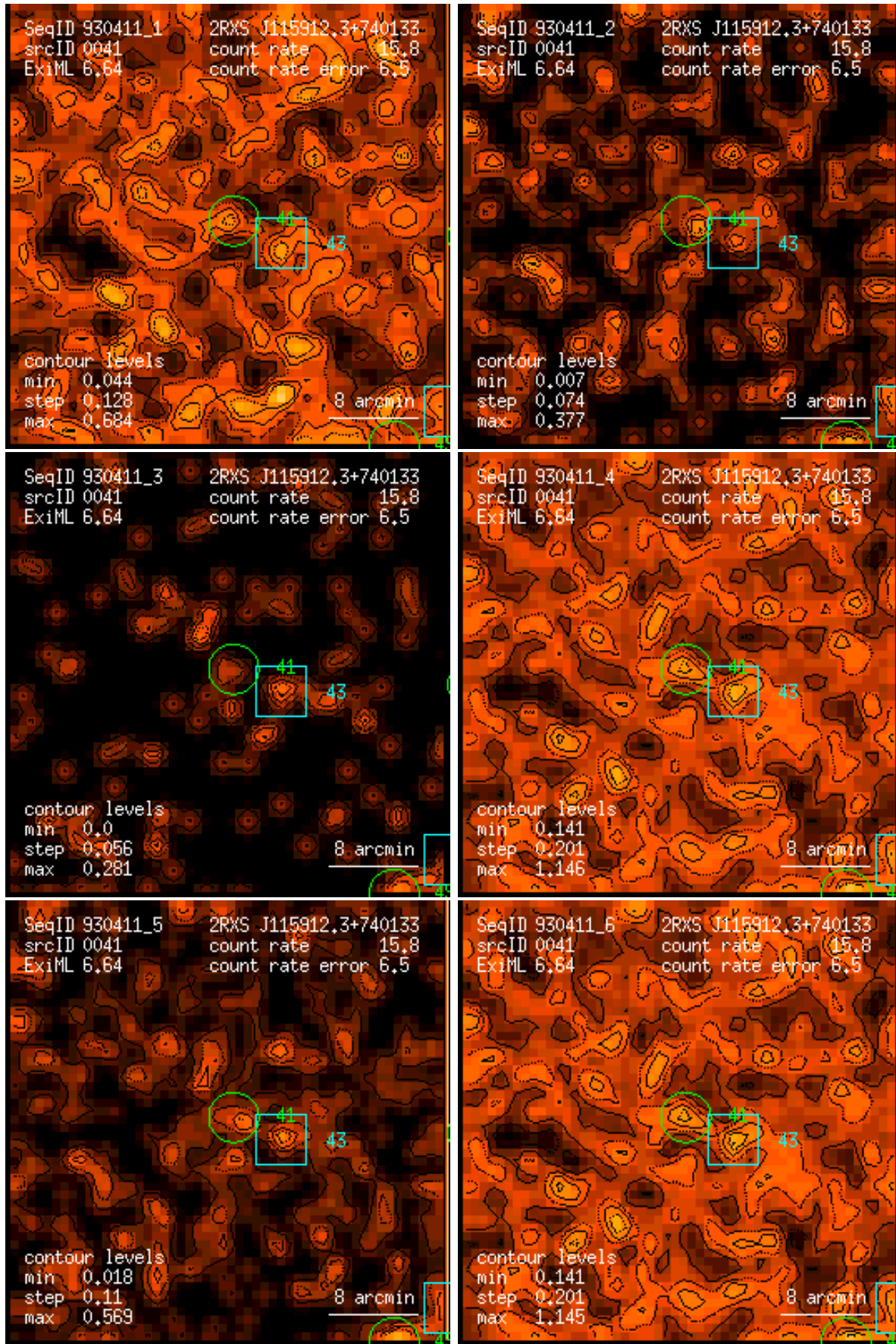
Figure 41: RASS 930411: detection 0041: band rate images, Gaussian filter: (1) PSPC channels 11 – 41, (2) 52 – 90, (3) 91 – 201, (4) 11 – 235, (5) 52 – 201, (6) 11 – 201. Broad band rates in counts/ks. Band rate contour levels in counts/ks/arcmin 2 .
