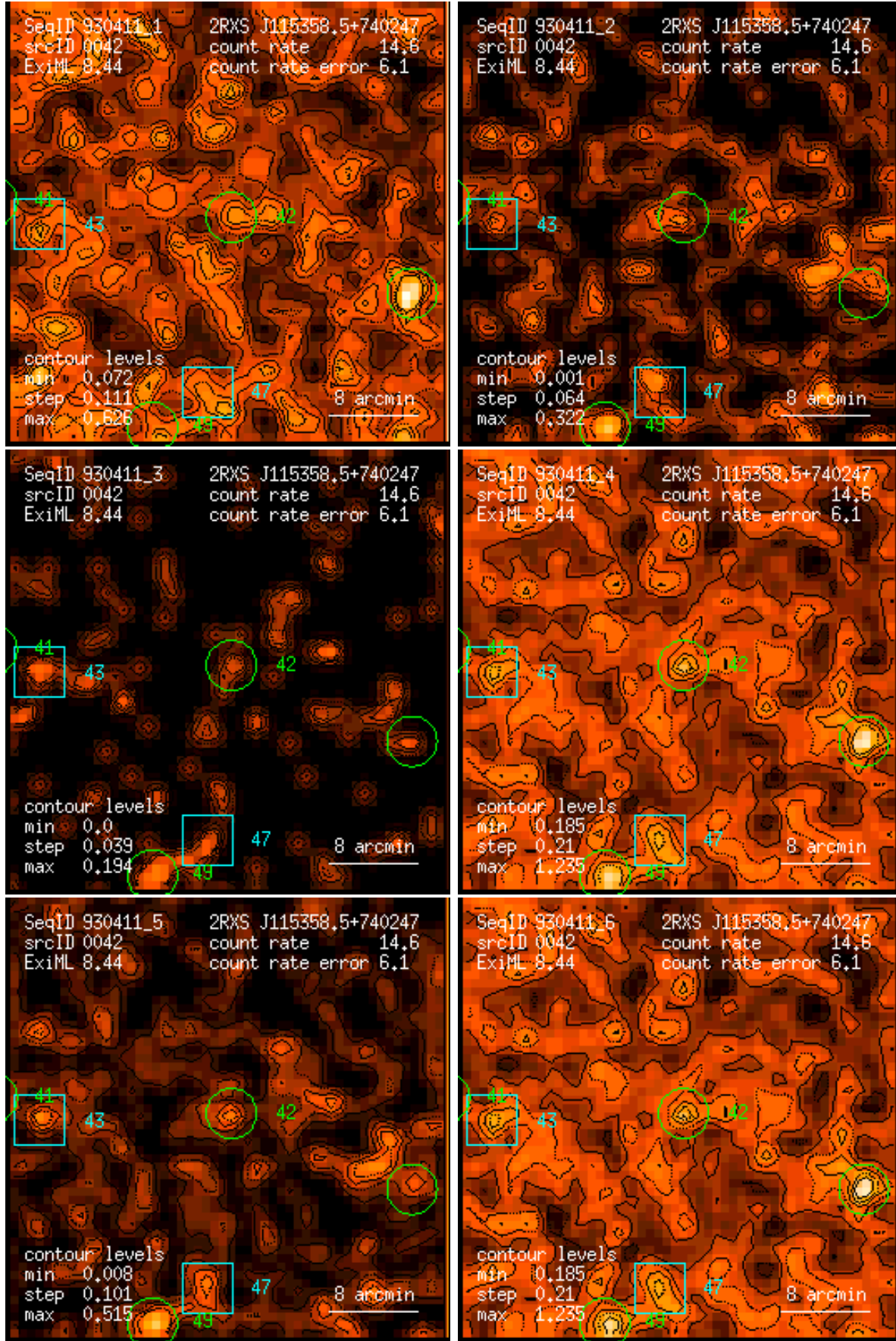
Figure 42: RASS 930411: detection 0042: band rate images, Gaussian filter: (1) PSPC channels 11 – 41, (2) 52 – 90, (3) 91 – 201, (4) 11 – 235, (5) 52 – 201, (6) 11 – 201. Broad band rates in counts/ks. Band rate contour levels in counts/ks/arcmin 2 .
