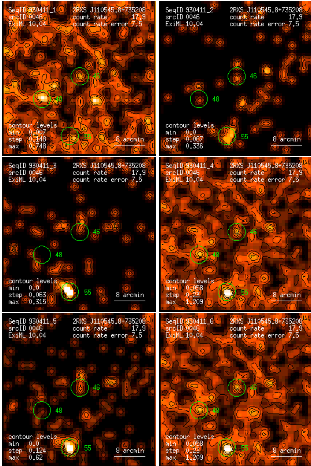
Figure 46: RASS 930411: detection 0046: band rate images, Gaussian filter: (1) PSPC channels 11 – 41, (2) 52 – 90, (3) 91 – 201, (4) 11 – 235, (5) 52 – 201, (6) 11 – 201. Broad band rates in counts/ks. Band rate contour levels in counts/ks/arcmin 2 .
