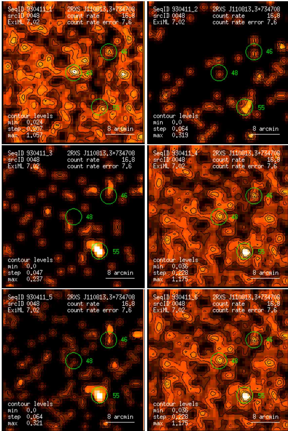
Figure 48: RASS 930411: detection 0048: band rate images, Gaussian filter: (1) PSPC channels 11 – 41, (2) 52 – 90, (3) 91 – 201, (4) 11 – 235, (5) 52 – 201, (6) 11 – 201. Broad band rates in counts/ks. Band rate contour levels in counts/ks/arcmin 2 .
