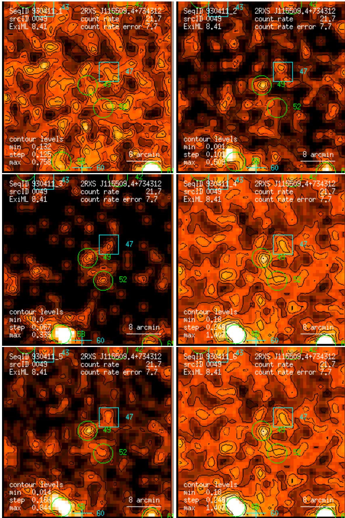
Figure 49: RASS 930411: detection 0049: band rate images, Gaussian filter: (1) PSPC channels 11 – 41, (2) 52 – 90, (3) 91 – 201, (4) 11 – 235, (5) 52 – 201, (6) 11 – 201. Broad band rates in counts/ks. Band rate contour levels in counts/ks/arcmin 2 .
