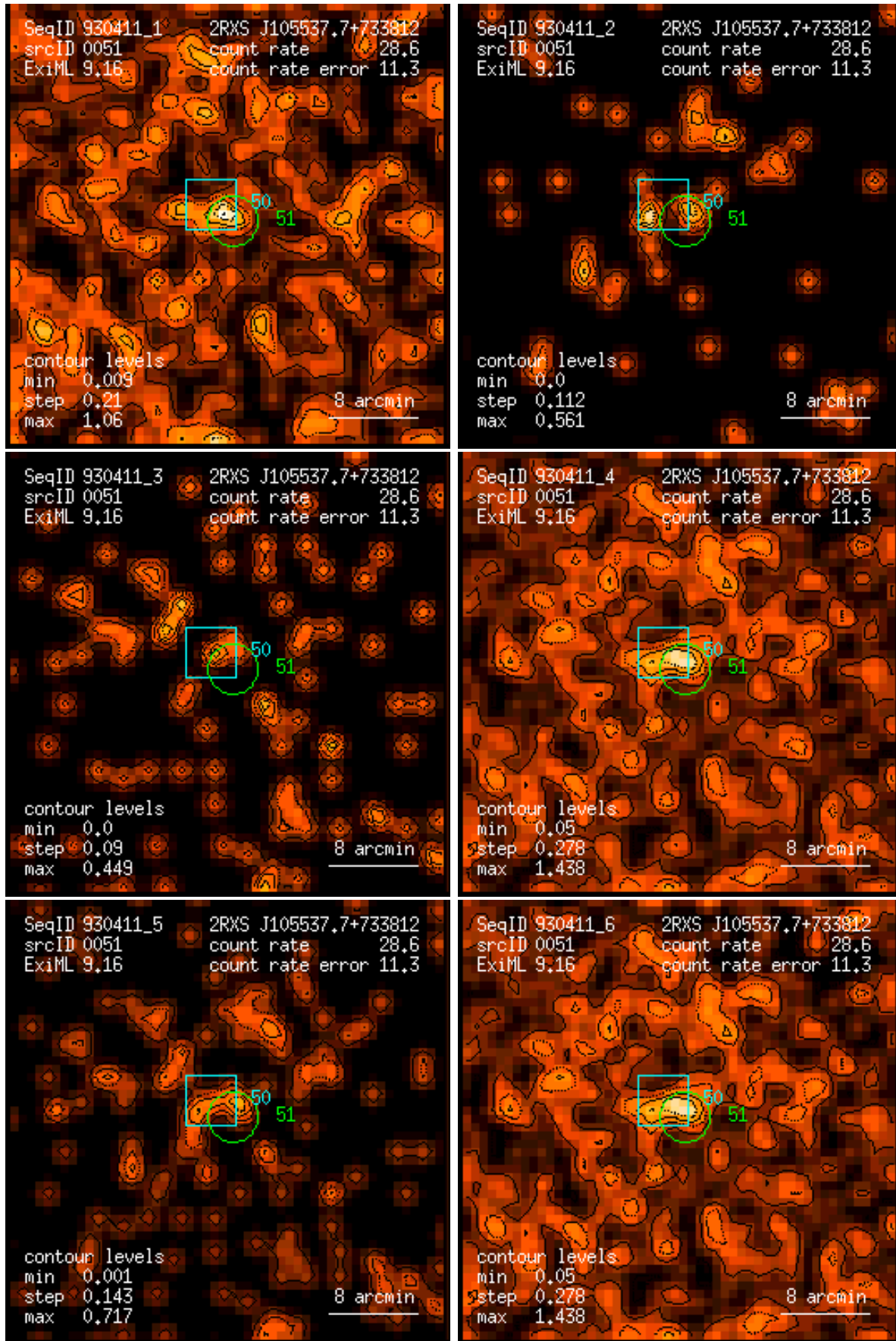
Figure 51: RASS 930411: detection 0051: band rate images, Gaussian filter: (1) PSPC channels 11 – 41, (2) 52 – 90, (3) 91 – 201, (4) 11 – 235, (5) 52 – 201, (6) 11 – 201. Broad band rates in counts/ks. Band rate contour levels in counts/ks/arcmin 2 .
