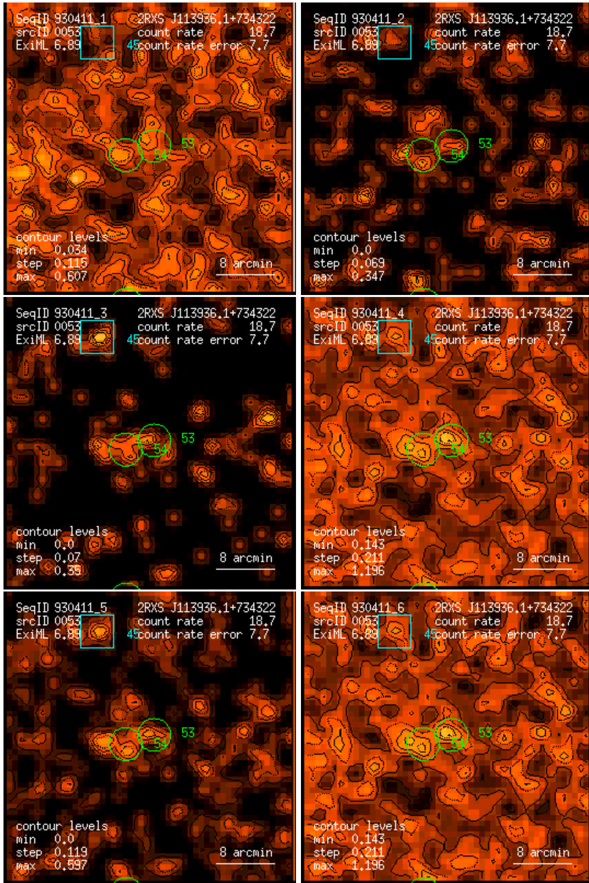
Figure 53: RASS 930411: detection 0053: band rate images, Gaussian filter: (1) PSPC channels 11 – 41, (2) 52 – 90, (3) 91 – 201, (4) 11 – 235, (5) 52 – 201, (6) 11 – 201. Broad band rates in counts/ks. Band rate contour levels in counts/ks/arcmin 2 .
