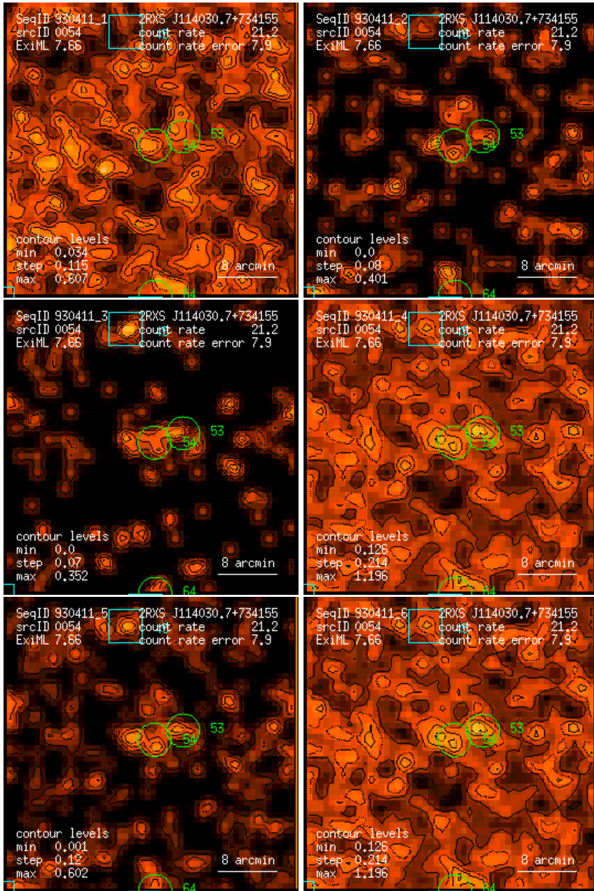
Figure 54: RASS 930411: detection 0054: band rate images, Gaussian filter: (1) PSPC channels 11 – 41, (2) 52 – 90, (3) 91 – 201, (4) 11 – 235, (5) 52 – 201, (6) 11 – 201. Broad band rates in counts/ks. Band rate contour levels in counts/ks/arcmin 2 .
