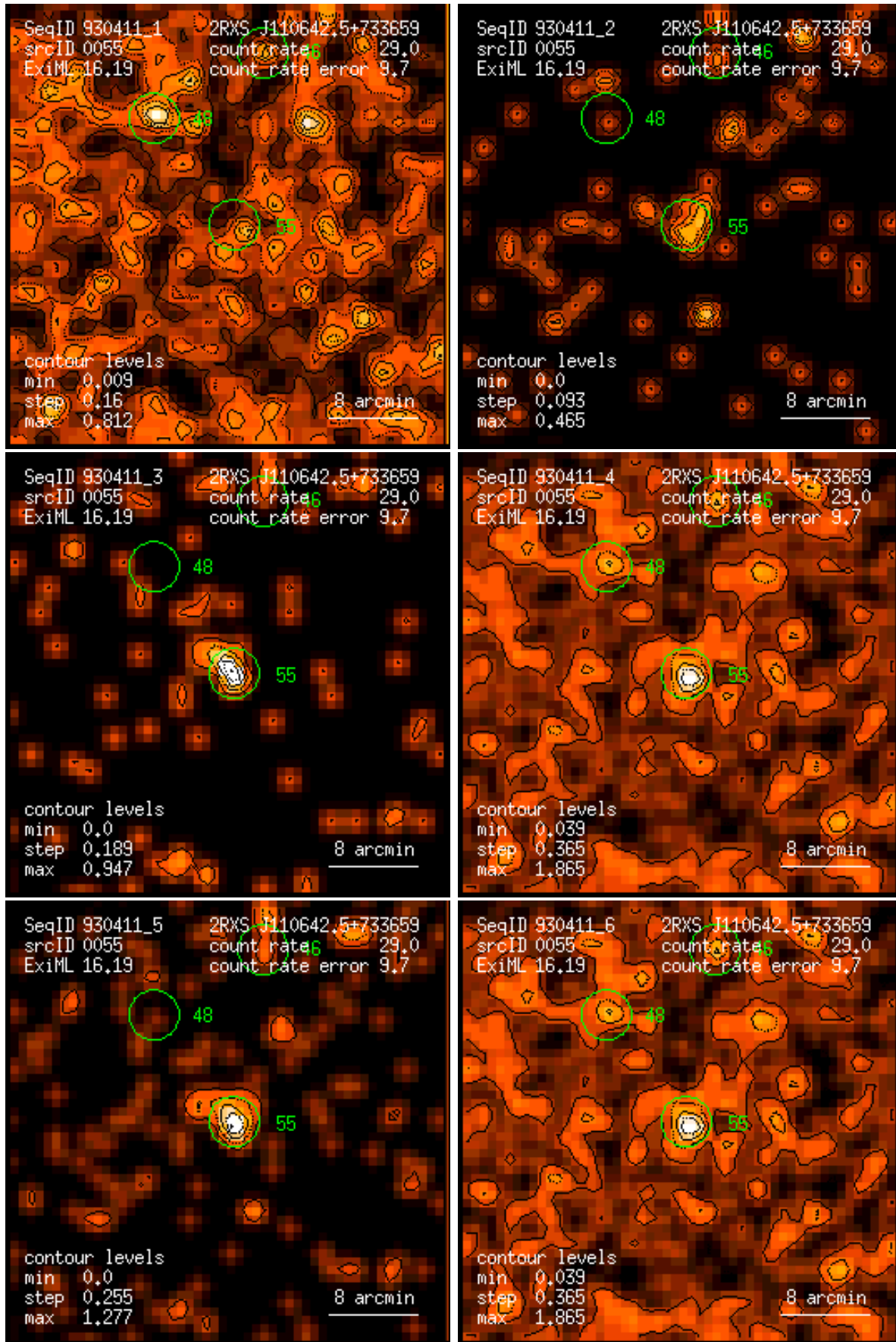
Figure 55: RASS 930411: detection 0055: band rate images, Gaussian filter: (1) PSPC channels 11 – 41, (2) 52 – 90, (3) 91 – 201, (4) 11 – 235, (5) 52 – 201, (6) 11 – 201. Broad band rates in counts/ks. Band rate contour levels in counts/ks/arcmin 2 .
