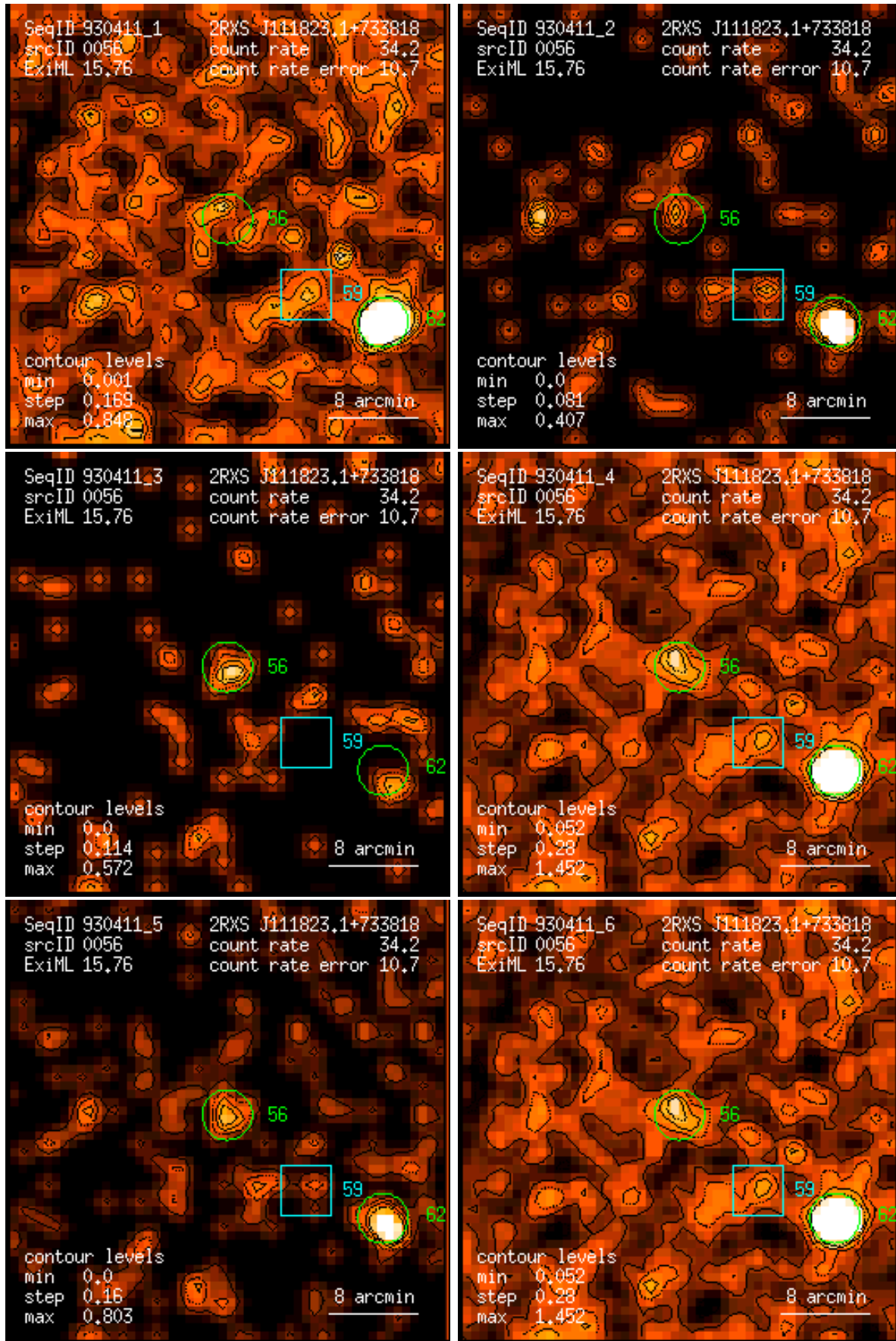
Figure 56: RASS 930411: detection 0056: band rate images, Gaussian filter: (1) PSPC channels 11 – 41, (2) 52 – 90, (3) 91 – 201, (4) 11 – 235, (5) 52 – 201, (6) 11 – 201. Broad band rates in counts/ks. Band rate contour levels in counts/ks/arcmin 2 .
