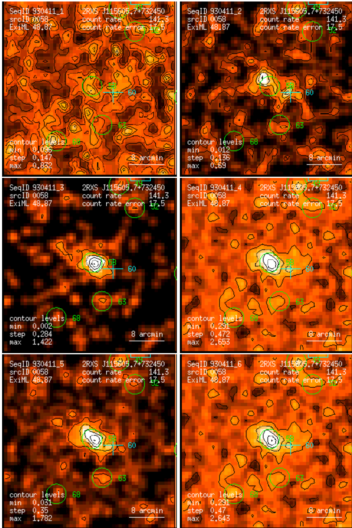
Figure 58: RASS 930411: detection 0058: band rate images, Gaussian filter: (1) PSPC channels 11 – 41, (2) 52 – 90, (3) 91 – 201, (4) 11 – 235, (5) 52 – 201, (6) 11 – 201. Broad band rates in counts/ks. Band rate contour levels in counts/ks/arcmin 2 .
