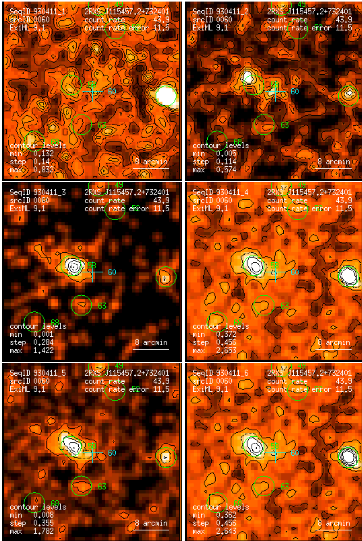
Figure 60: RASS 930411: detection 0060: band rate images, Gaussian filter: (1) PSPC channels 11 – 41, (2) 52 – 90, (3) 91 – 201, (4) 11 – 235, (5) 52 – 201, (6) 11 – 201. Broad band rates in counts/ks. Band rate contour levels in counts/ks/arcmin 2 .
