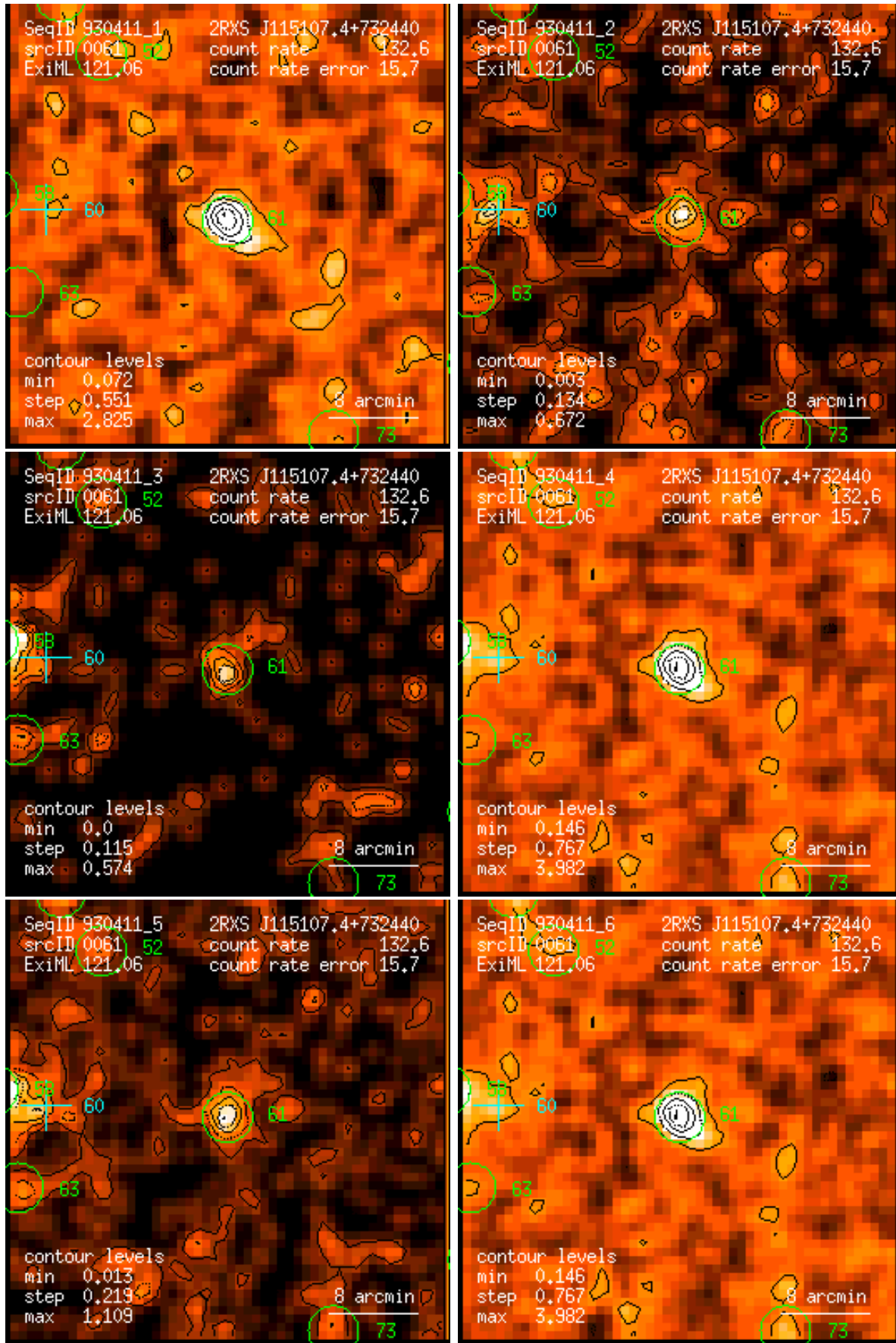
Figure 61: RASS 930411: detection 0061: band rate images, Gaussian filter: (1) PSPC channels 11 – 41, (2) 52 – 90, (3) 91 – 201, (4) 11 – 235, (5) 52 – 201, (6) 11 – 201. Broad band rates in counts/ks. Band rate contour levels in counts/ks/arcmin 2 .
