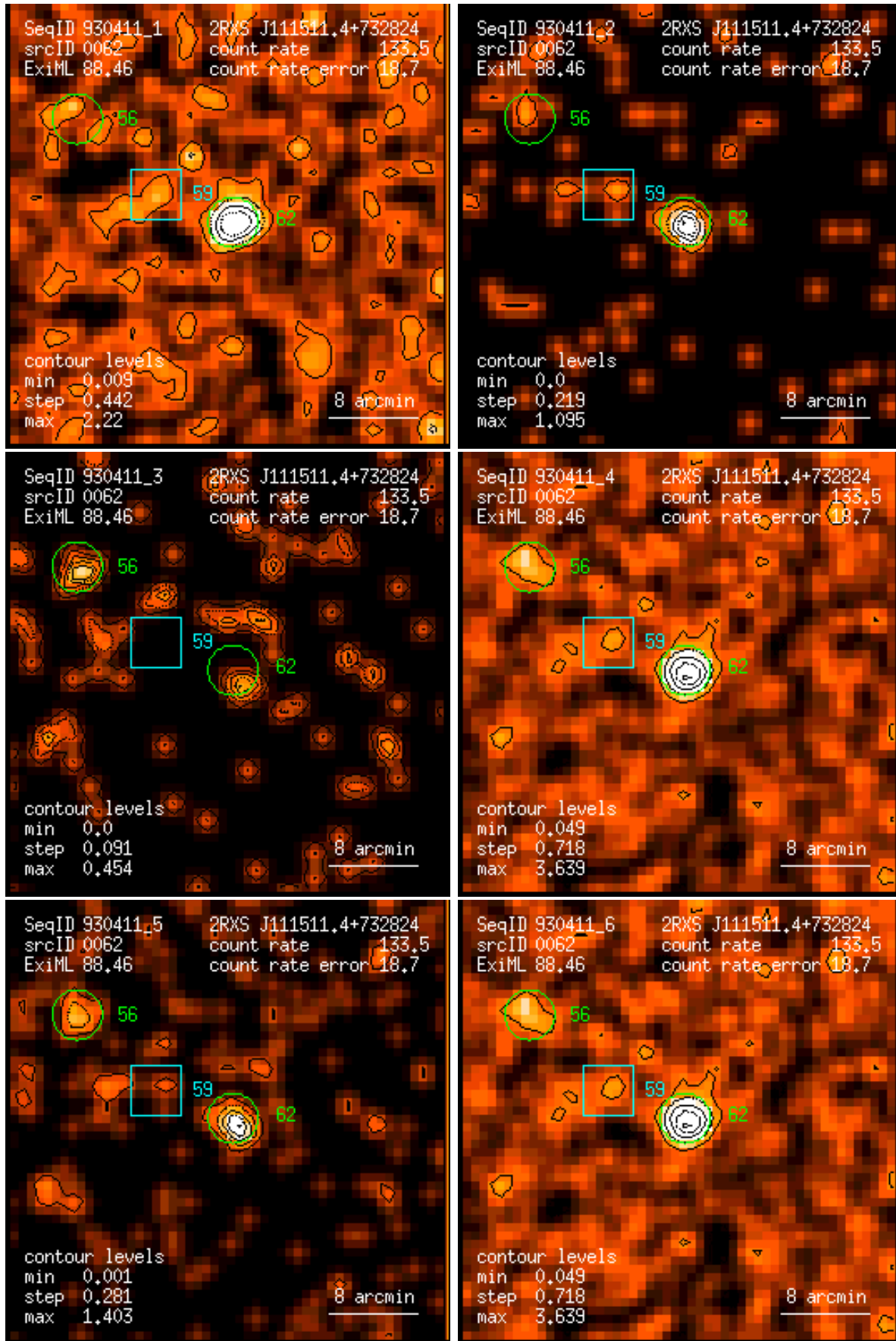
Figure 62: RASS 930411: detection 0062: band rate images, Gaussian filter: (1) PSPC channels 11 – 41, (2) 52 – 90, (3) 91 – 201, (4) 11 – 235, (5) 52 – 201, (6) 11 – 201. Broad band rates in counts/ks. Band rate contour levels in counts/ks/arcmin 2 .
