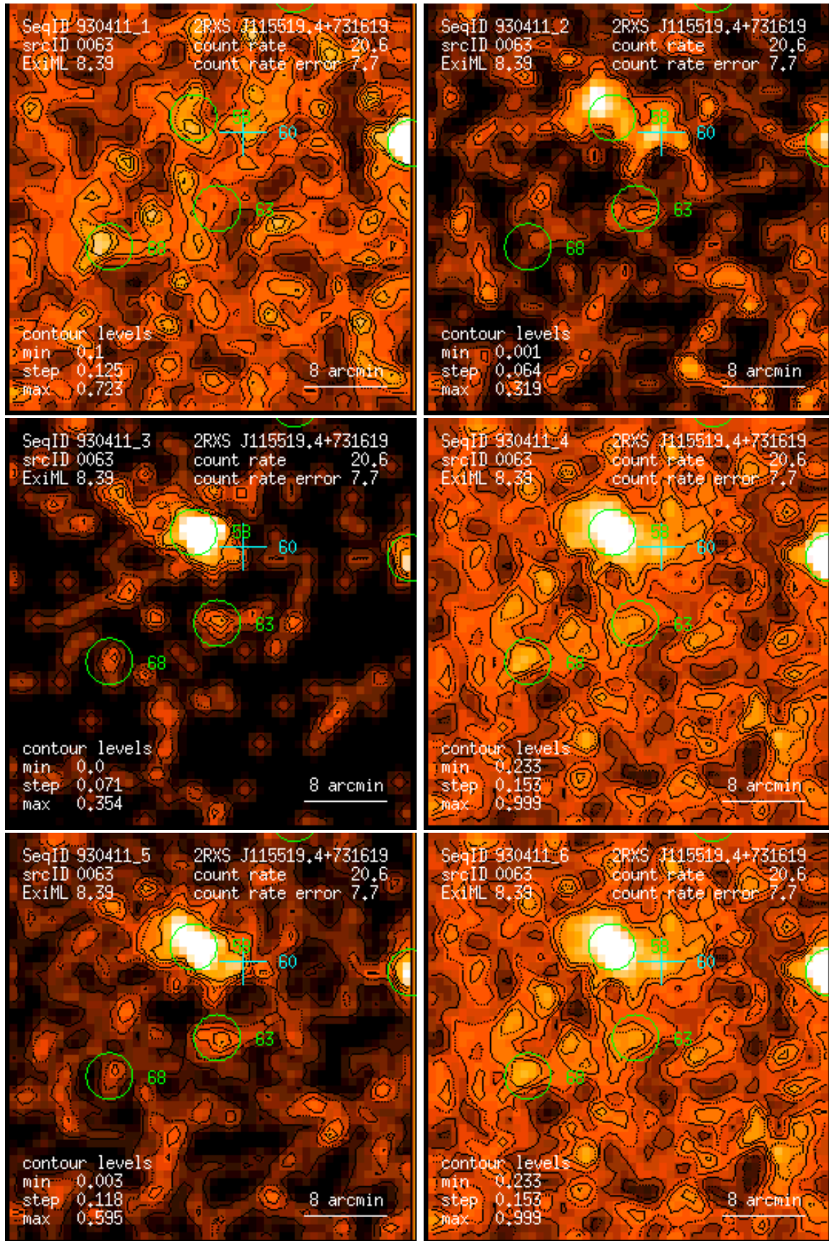
Figure 63: RASS 930411: detection 0063: band rate images, Gaussian filter: (1) PSPC channels 11 – 41, (2) 52 – 90, (3) 91 – 201, (4) 11 – 235, (5) 52 – 201, (6) 11 – 201. Broad band rates in counts/ks. Band rate contour levels in counts/ks/arcmin 2 .
