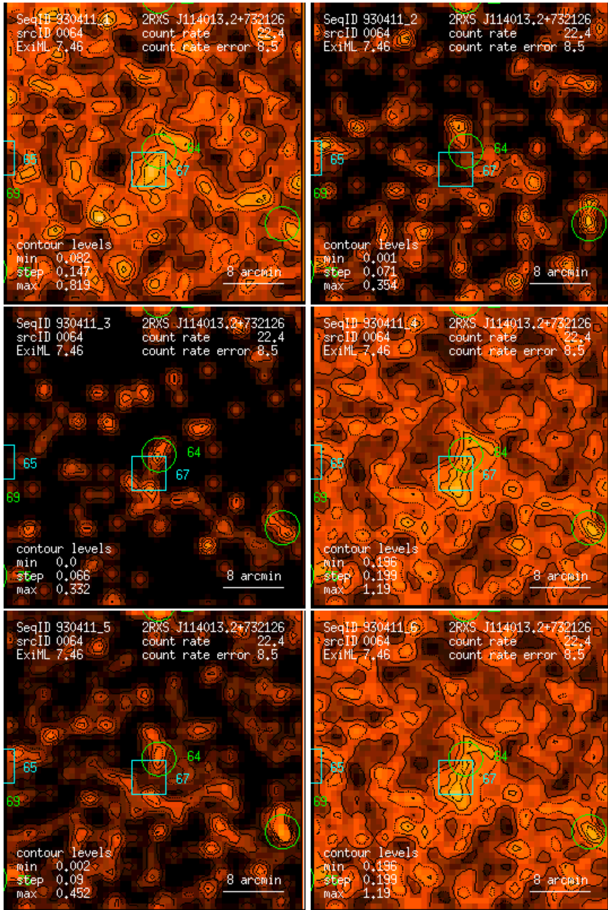
Figure 64: RASS 930411: detection 0064: band rate images, Gaussian filter: (1) PSPC channels 11 – 41, (2) 52 – 90, (3) 91 – 201, (4) 11 – 235, (5) 52 – 201, (6) 11 – 201. Broad band rates in counts/ks. Band rate contour levels in counts/ks/arcmin 2 .
