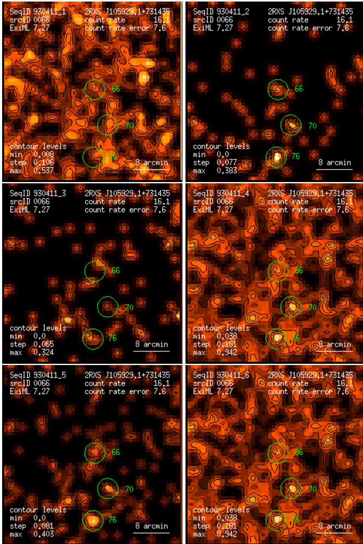
Figure 66: RASS 930411: detection 0066: band rate images, Gaussian filter: (1) PSPC channels 11 – 41, (2) 52 – 90, (3) 91 – 201, (4) 11 – 235, (5) 52 – 201, (6) 11 – 201. Broad band rates in counts/ks. Band rate contour levels in counts/ks/arcmin 2 .
