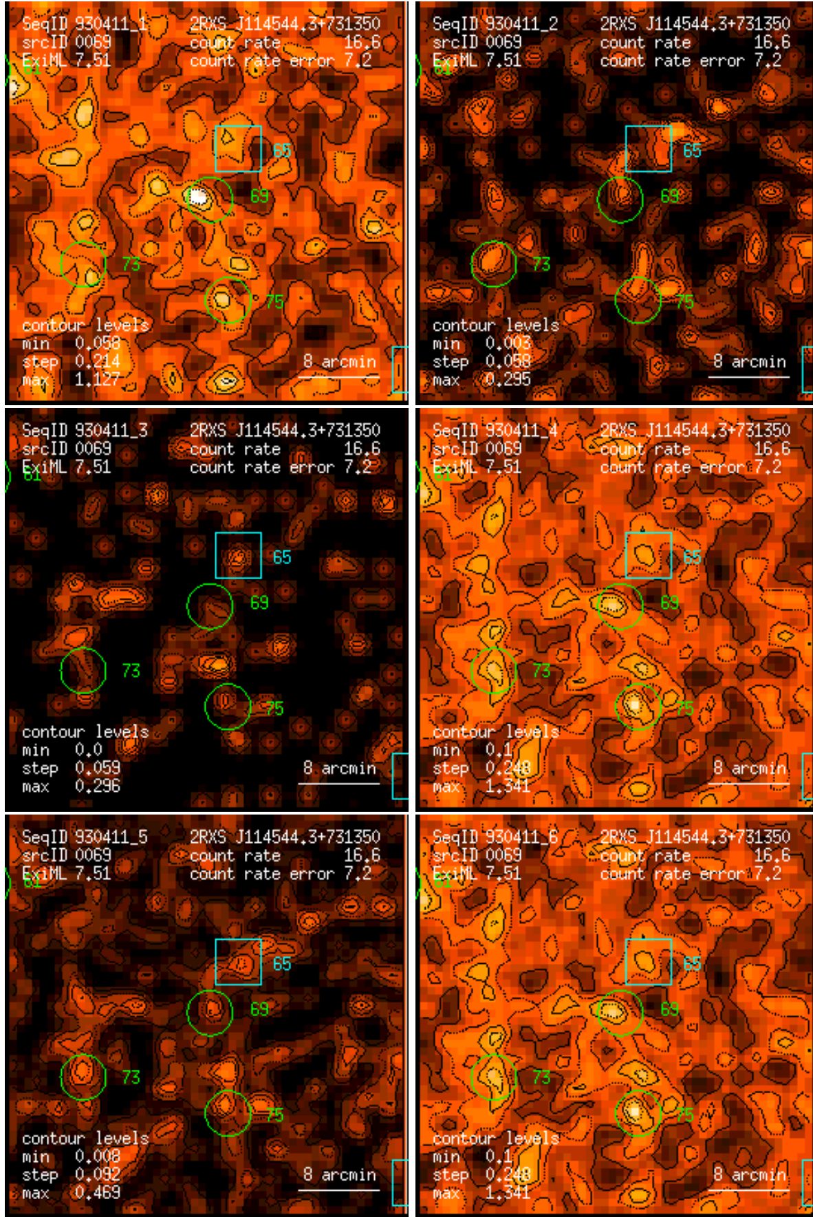
Figure 69: RASS 930411: detection 0069: band rate images, Gaussian filter: (1) PSPC channels 11 – 41, (2) 52 – 90, (3) 91 – 201, (4) 11 – 235, (5) 52 – 201, (6) 11 – 201. Broad band rates in counts/ks. Band rate contour levels in counts/ks/arcmin 2 .
