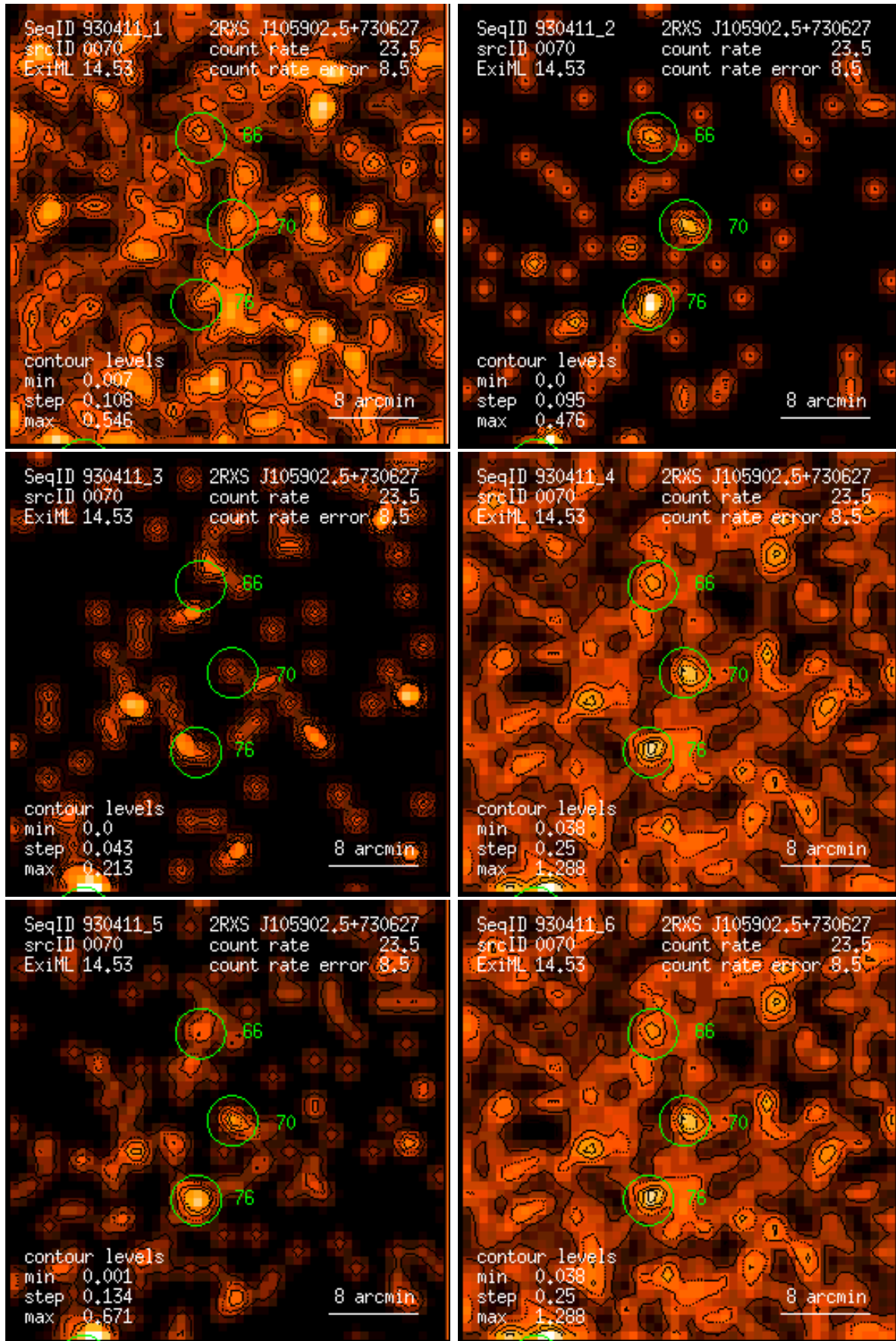
Figure 70: RASS 930411: detection 0070: band rate images, Gaussian filter: (1) PSPC channels 11 – 41, (2) 52 – 90, (3) 91 – 201, (4) 11 – 235, (5) 52 – 201, (6) 11 – 201. Broad band rates in counts/ks. Band rate contour levels in counts/ks/arcmin 2 .
