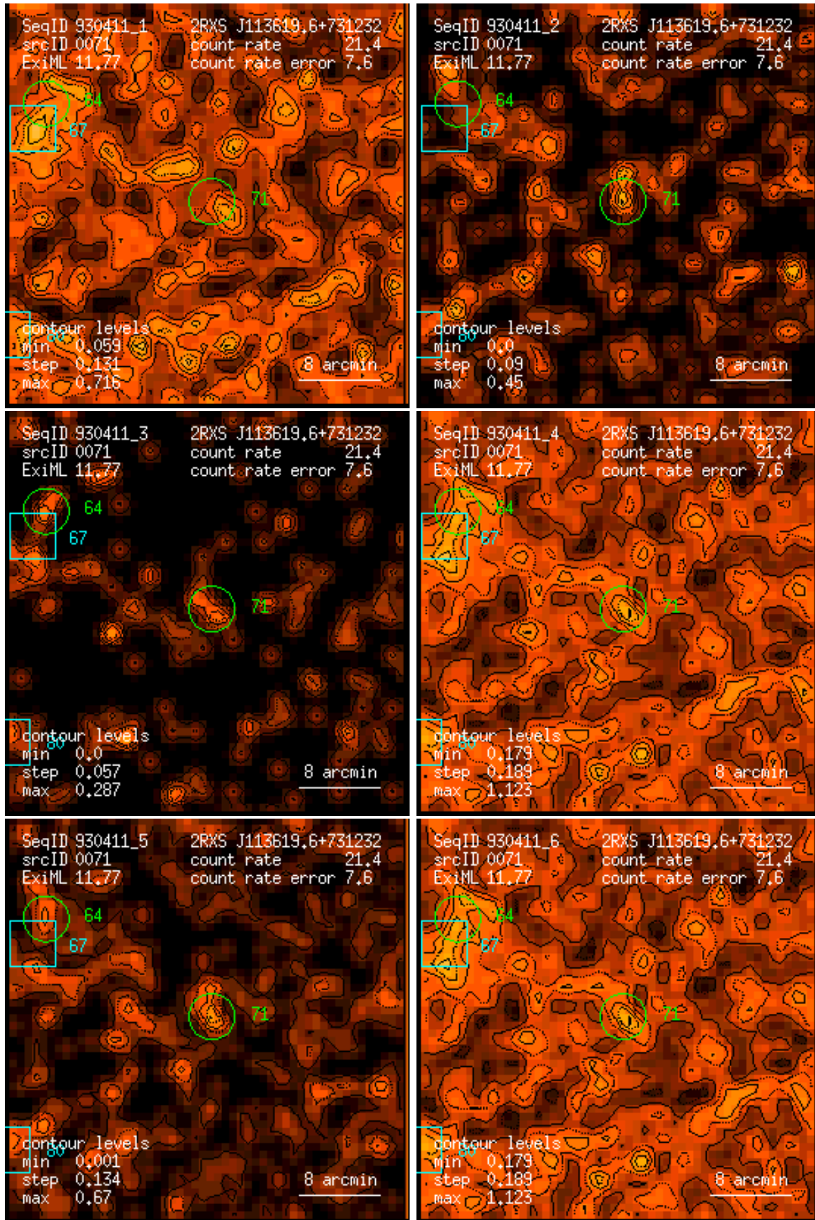
Figure 71: RASS 930411: detection 0071: band rate images, Gaussian filter: (1) PSPC channels 11 – 41, (2) 52 – 90, (3) 91 – 201, (4) 11 – 235, (5) 52 – 201, (6) 11 – 201. Broad band rates in counts/ks. Band rate contour levels in counts/ks/arcmin 2 .
