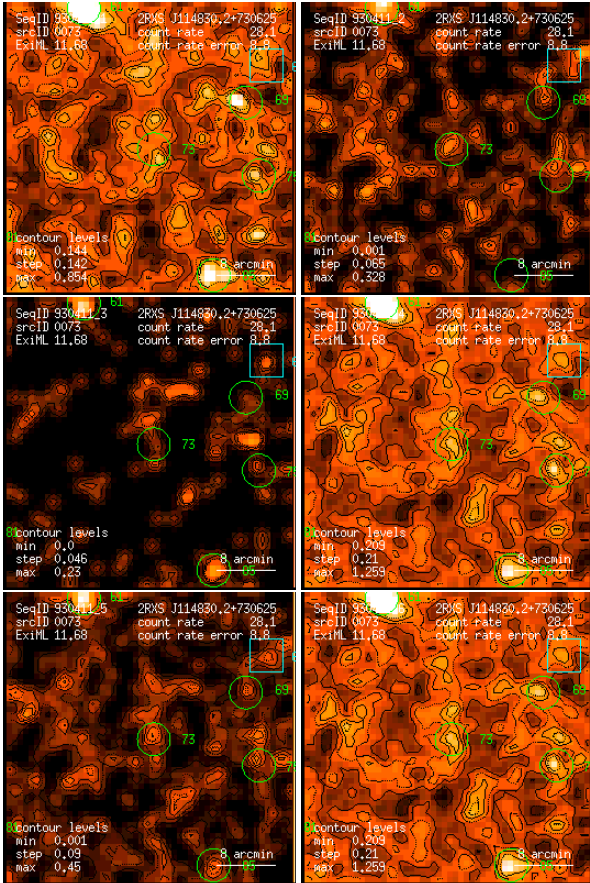
Figure 73: RASS 930411: detection 0073: band rate images, Gaussian filter: (1) PSPC channels 11 – 41, (2) 52 – 90, (3) 91 – 201, (4) 11 – 235, (5) 52 – 201, (6) 11 – 201. Broad band rates in counts/ks. Band rate contour levels in counts/ks/arcmin 2 .
