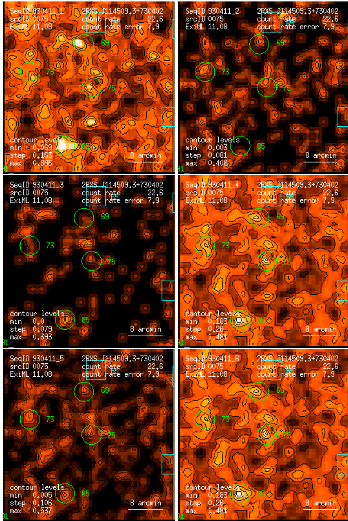
Figure 75: RASS 930411: detection 0075: band rate images, Gaussian filter: (1) PSPC channels 11 – 41, (2) 52 – 90, (3) 91 – 201, (4) 11 – 235, (5) 52 – 201, (6) 11 – 201. Broad band rates in counts/ks. Band rate contour levels in counts/ks/arcmin 2 .
