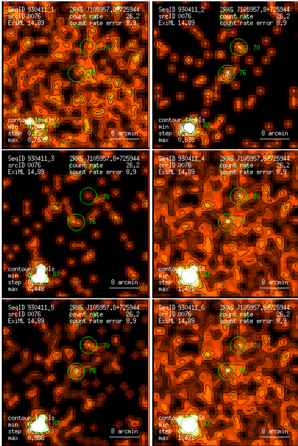
Figure 76: RASS 930411: detection 0076: band rate images, Gaussian filter: (1) PSPC channels 11 – 41, (2) 52 – 90, (3) 91 – 201, (4) 11 – 235, (5) 52 – 201, (6) 11 – 201. Broad band rates in counts/ks. Band rate contour levels in counts/ks/arcmin 2 .
