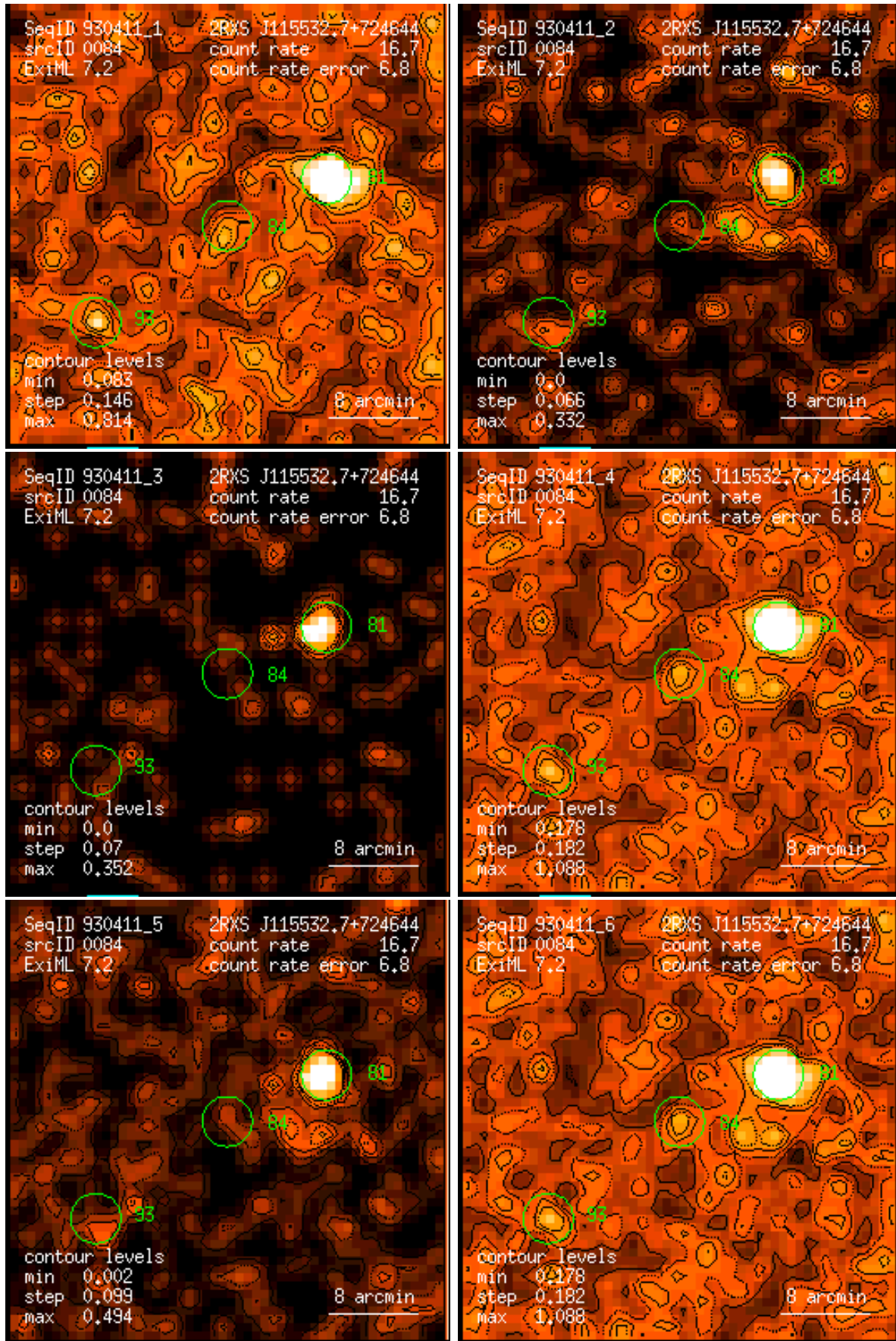
Figure 84: RASS 930411: detection 0084: band rate images, Gaussian filter: (1) PSPC channels 11 – 41, (2) 52 – 90, (3) 91 – 201, (4) 11 – 235, (5) 52 – 201, (6) 11 – 201. Broad band rates in counts/ks. Band rate contour levels in counts/ks/arcmin 2 .
