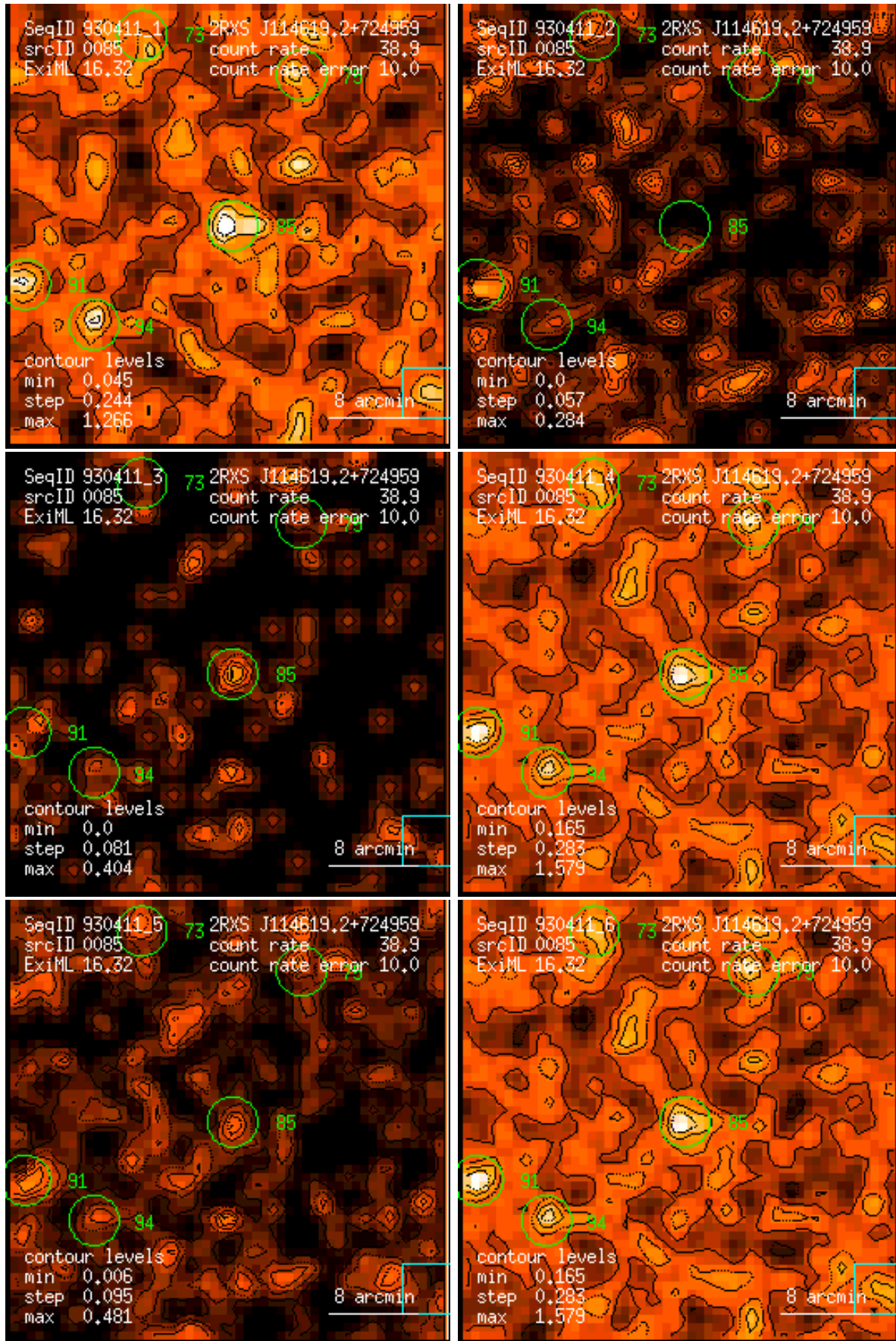
Figure 85: RASS 930411: detection 0085: band rate images, Gaussian filter: (1) PSPC channels 11 – 41, (2) 52 – 90, (3) 91 – 201, (4) 11 – 235, (5) 52 – 201, (6) 11 – 201. Broad band rates in counts/ks. Band rate contour levels in counts/ks/arcmin 2 .
