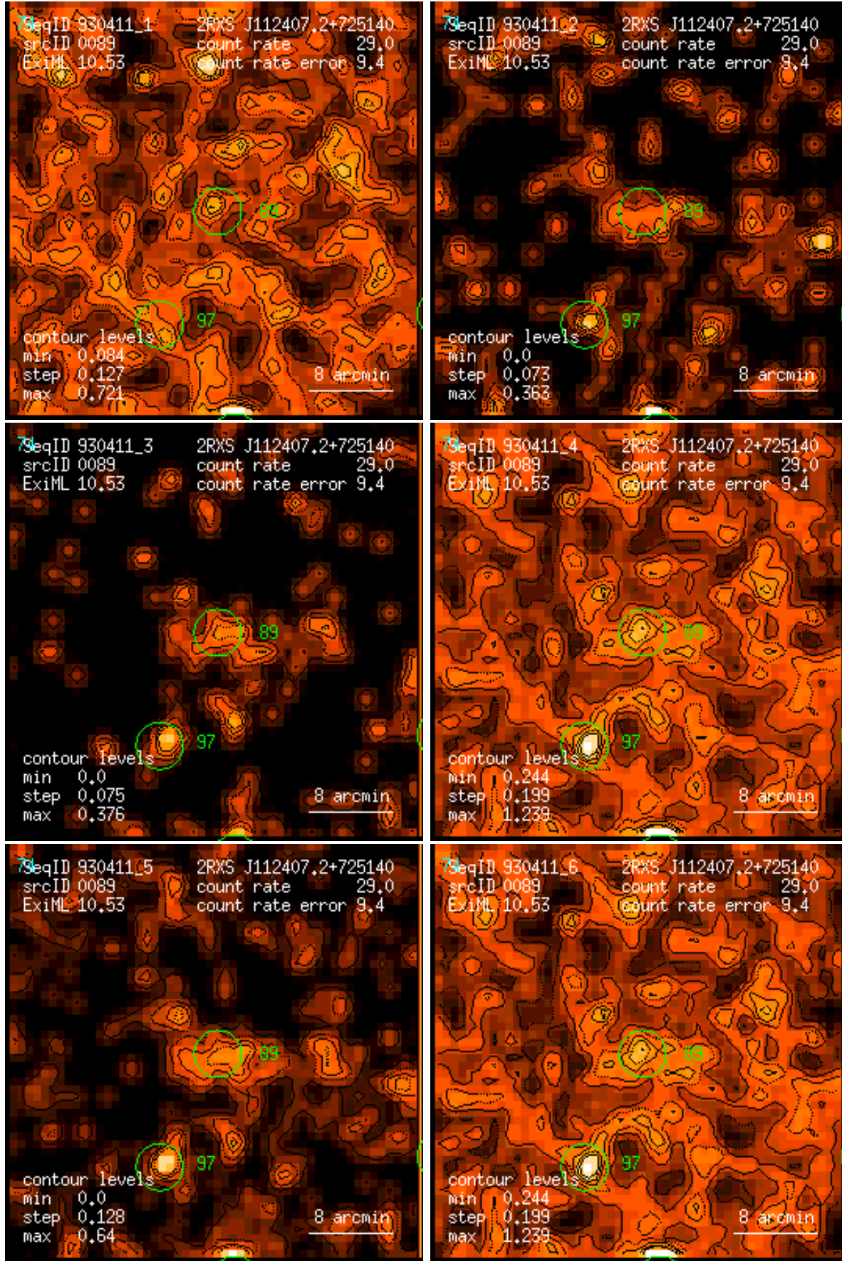
Figure 89: RASS 930411: detection 0089: band rate images, Gaussian filter: (1) PSPC channels 11 – 41, (2) 52 – 90, (3) 91 – 201, (4) 11 – 235, (5) 52 – 201, (6) 11 – 201. Broad band rates in counts/ks. Band rate contour levels in counts/ks/arcmin 2 .
