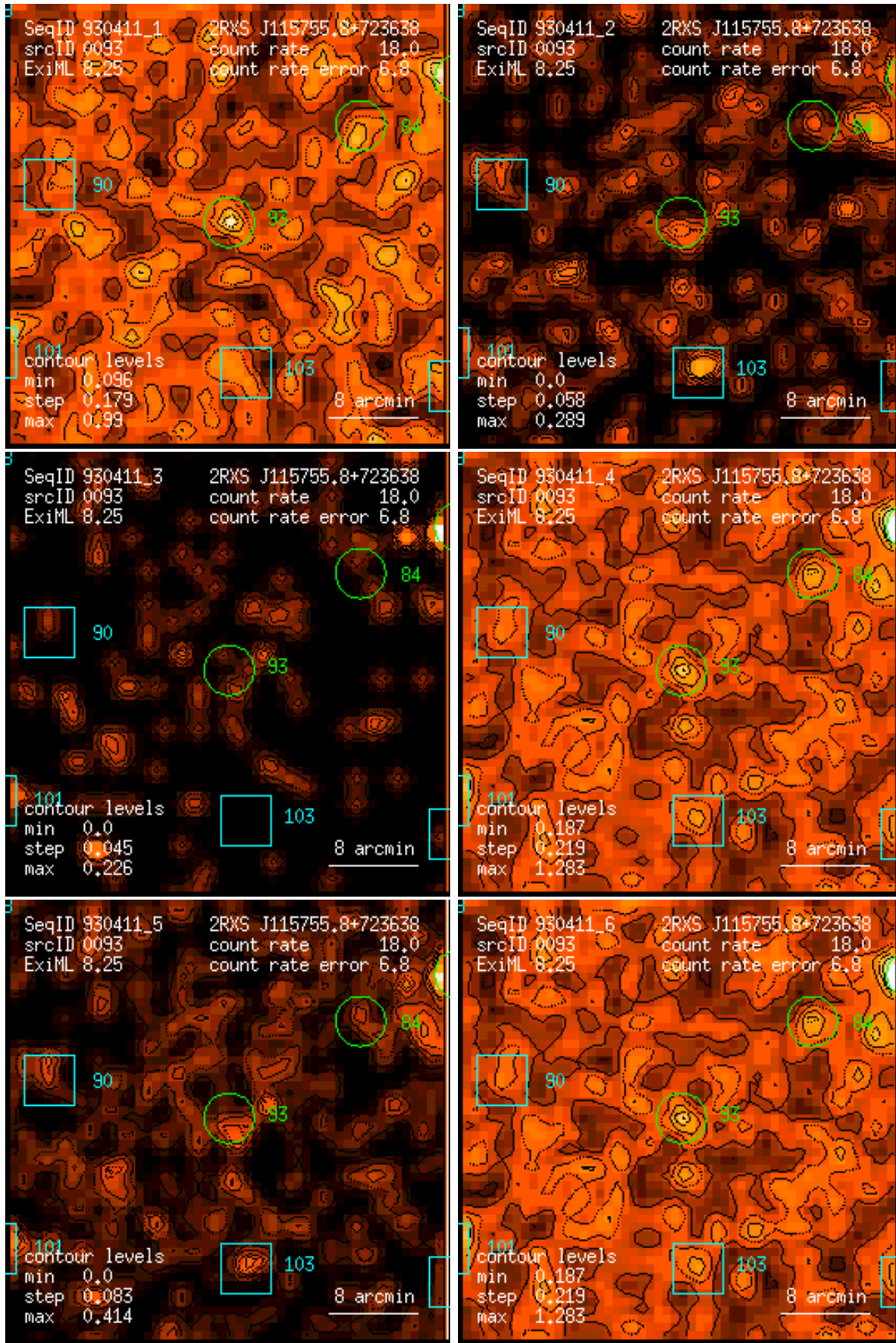
Figure 93: RASS 930411: detection 0093: band rate images, Gaussian filter: (1) PSPC channels 11 – 41, (2) 52 – 90, (3) 91 – 201, (4) 11 – 235, (5) 52 – 201, (6) 11 – 201. Broad band rates in counts/ks. Band rate contour levels in counts/ks/arcmin 2 .
