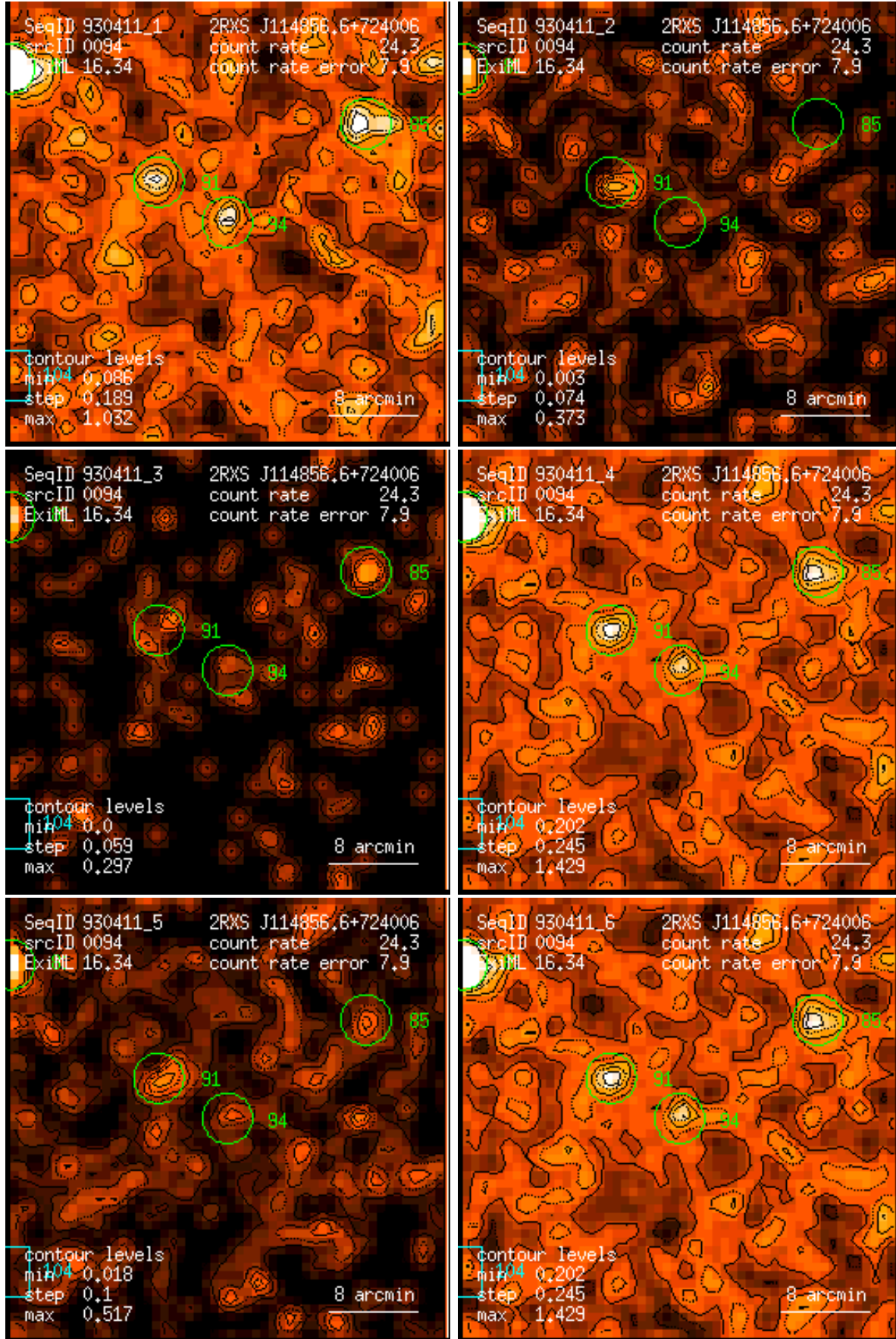
Figure 94: RASS 930411: detection 0094: band rate images, Gaussian filter: (1) PSPC channels 11 – 41, (2) 52 – 90, (3) 91 – 201, (4) 11 – 235, (5) 52 – 201, (6) 11 – 201. Broad band rates in counts/ks. Band rate contour levels in counts/ks/arcmin 2 .
