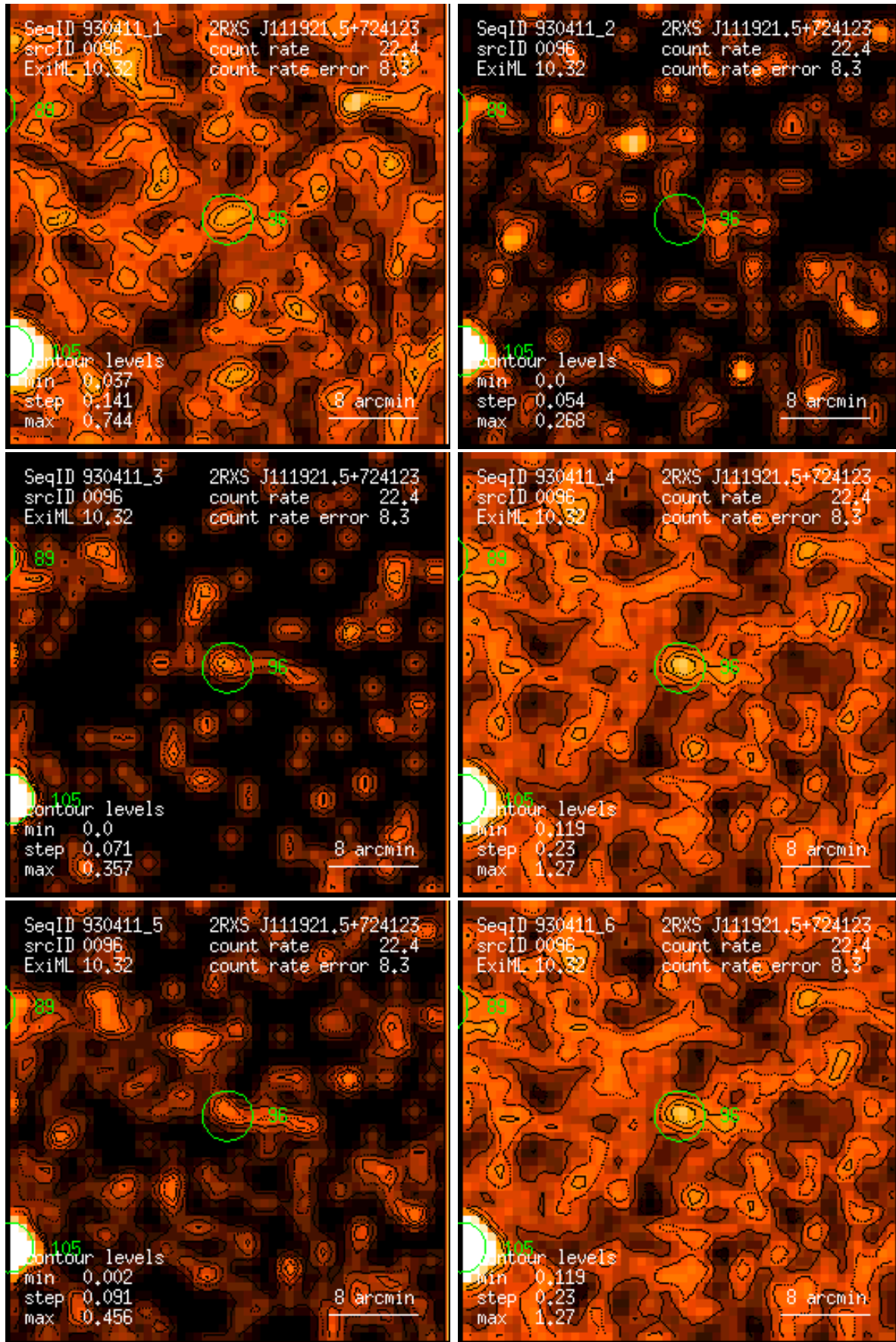
Figure 96: RASS 930411: detection 0096: band rate images, Gaussian filter: (1) PSPC channels 11 – 41, (2) 52 – 90, (3) 91 – 201, (4) 11 – 235, (5) 52 – 201, (6) 11 – 201. Broad band rates in counts/ks. Band rate contour levels in counts/ks/arcmin 2 .
