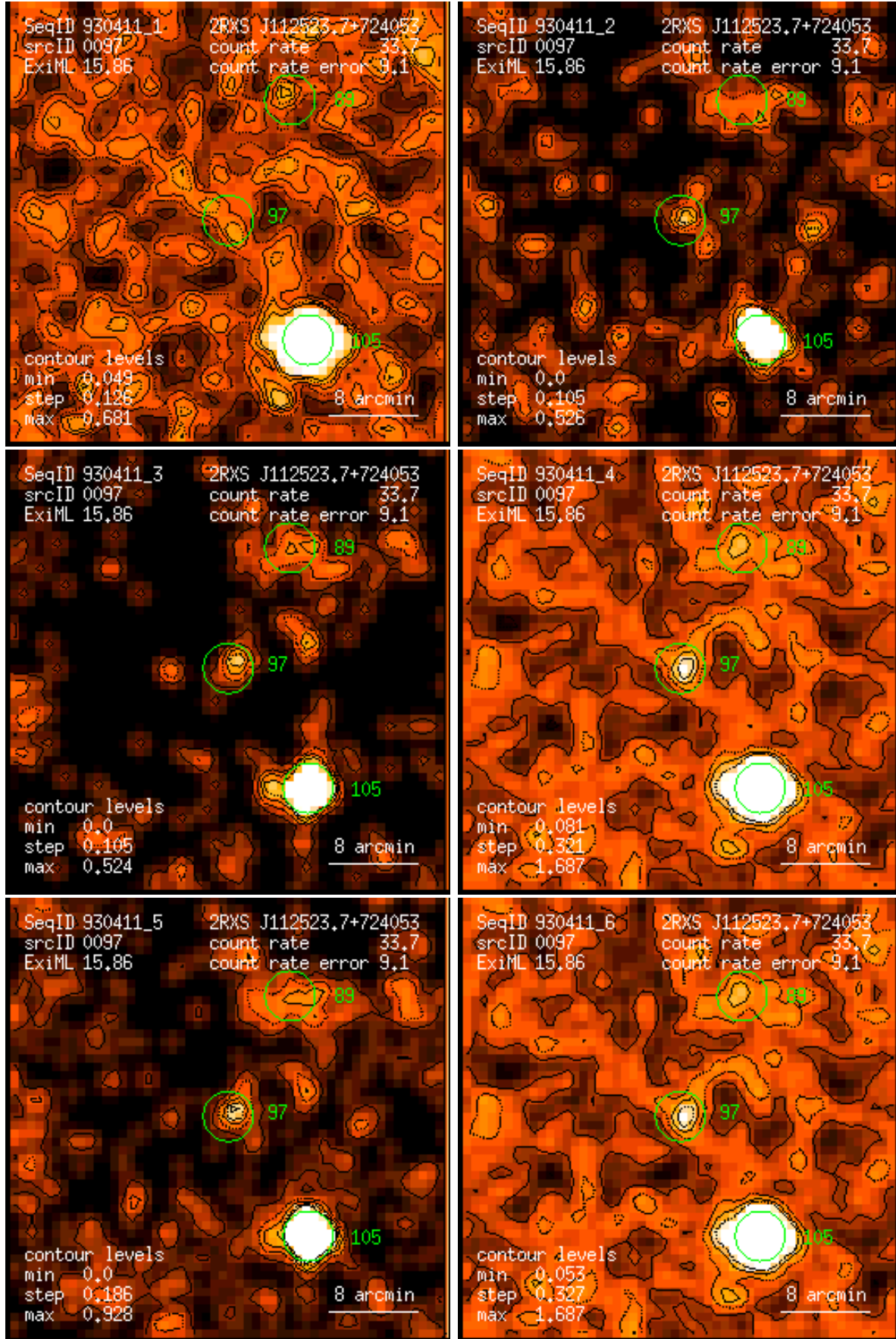
Figure 97: RASS 930411: detection 0097: band rate images, Gaussian filter: (1) PSPC channels 11 – 41, (2) 52 – 90, (3) 91 – 201, (4) 11 – 235, (5) 52 – 201, (6) 11 – 201. Broad band rates in counts/ks. Band rate contour levels in counts/ks/arcmin 2 .
