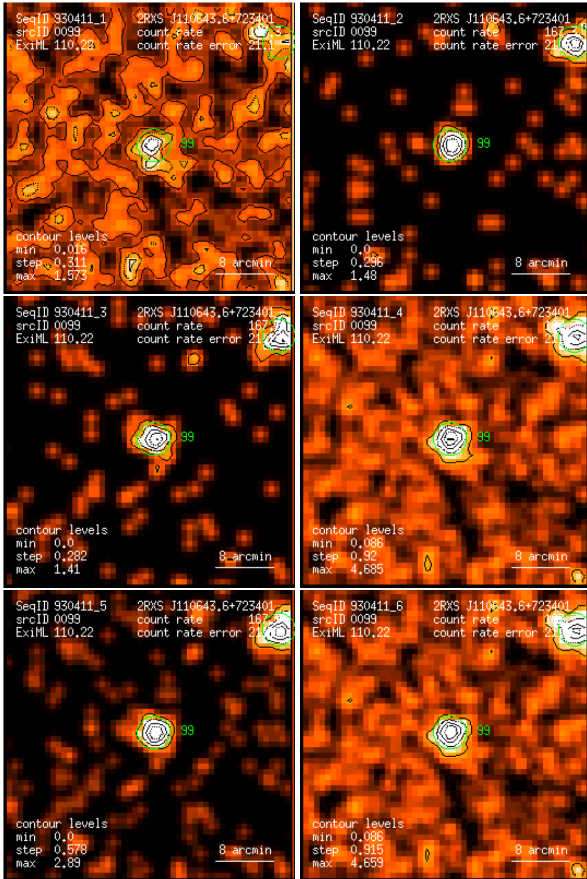
Figure 99: RASS 930411: detection 0099: band rate images, Gaussian filter: (1) PSPC channels 11 – 41, (2) 52 – 90, (3) 91 – 201, (4) 11 – 235, (5) 52 – 201, (6) 11 – 201. Broad band rates in counts/ks. Band rate contour levels in counts/ks/arcmin 2 .
